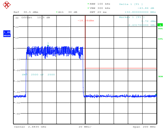
3DH1_Hopping_Upper
