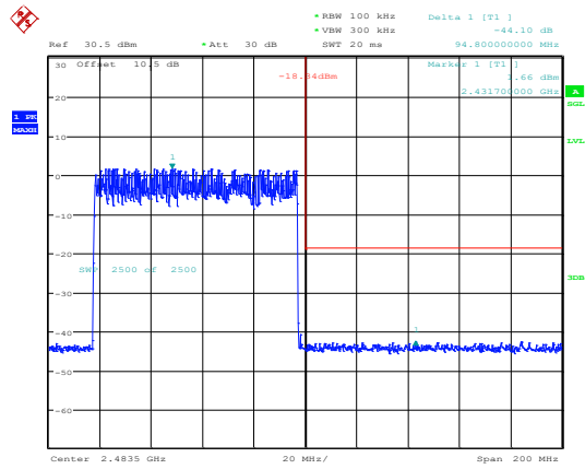
2DH1_Hopping_Upper
