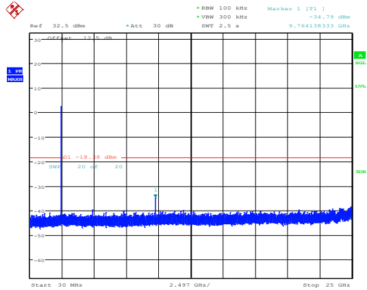
3DH1_Middle
