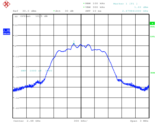
3DH1_High
