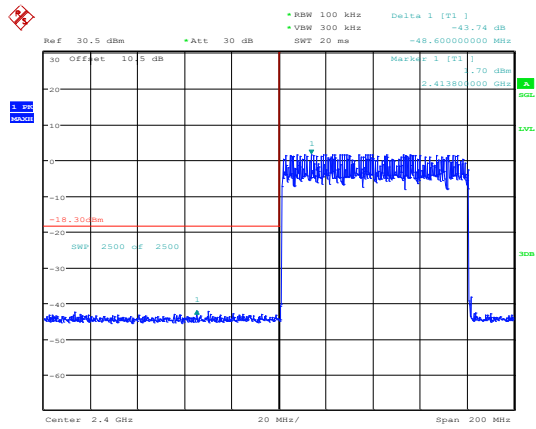
2DH1_Hopping_Lower
