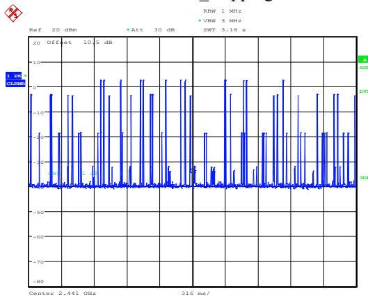
3DH5_Hopping
