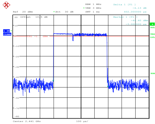
2DH1_Hopping
