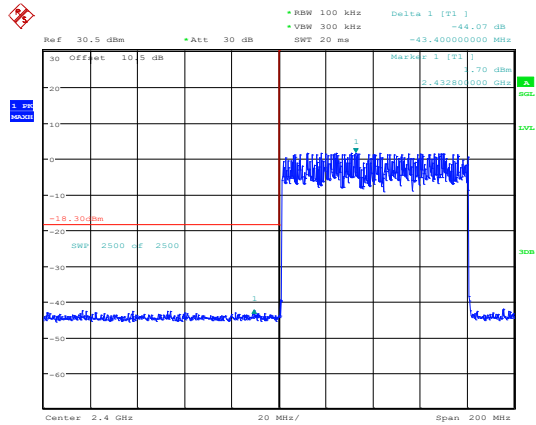
3DH1_Hopping_Lower
