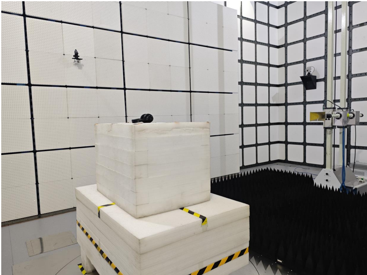
Radiated Emission 18-25GHz View
