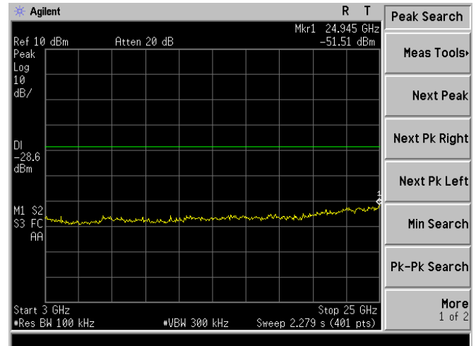
Low Channel 2407MHz
