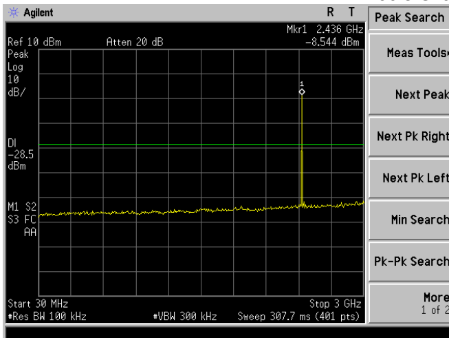
Middle Channel 2435MHz
