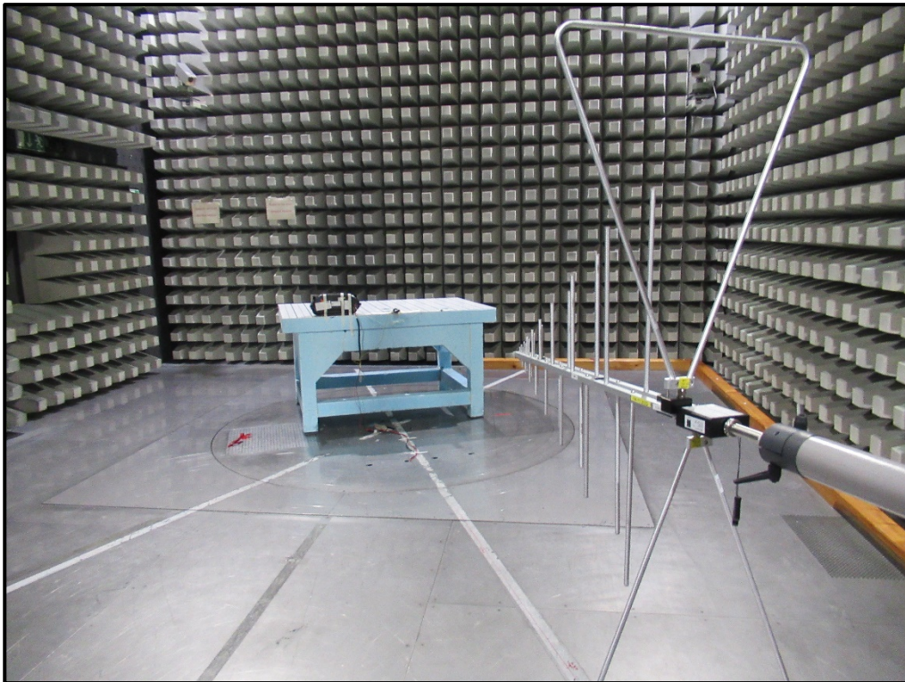
Photo 3: Radiated Spurious Emissions – 30 MHz to 1 GHz
