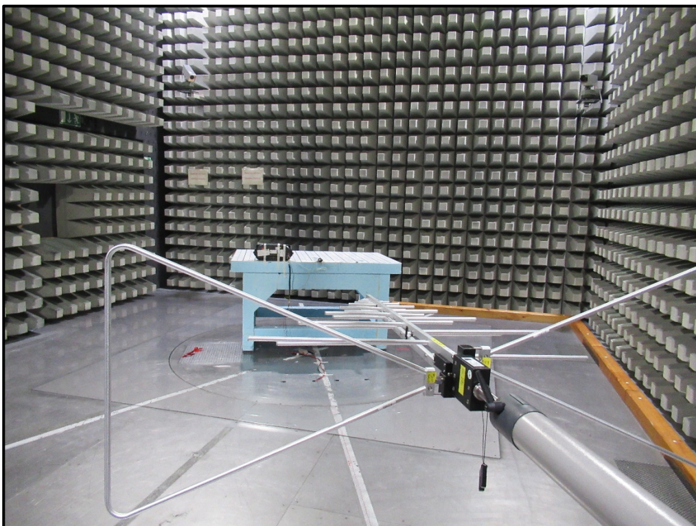
Photo 4: Radiated Spurious Emissions – 30 MHz to 1 GHz
