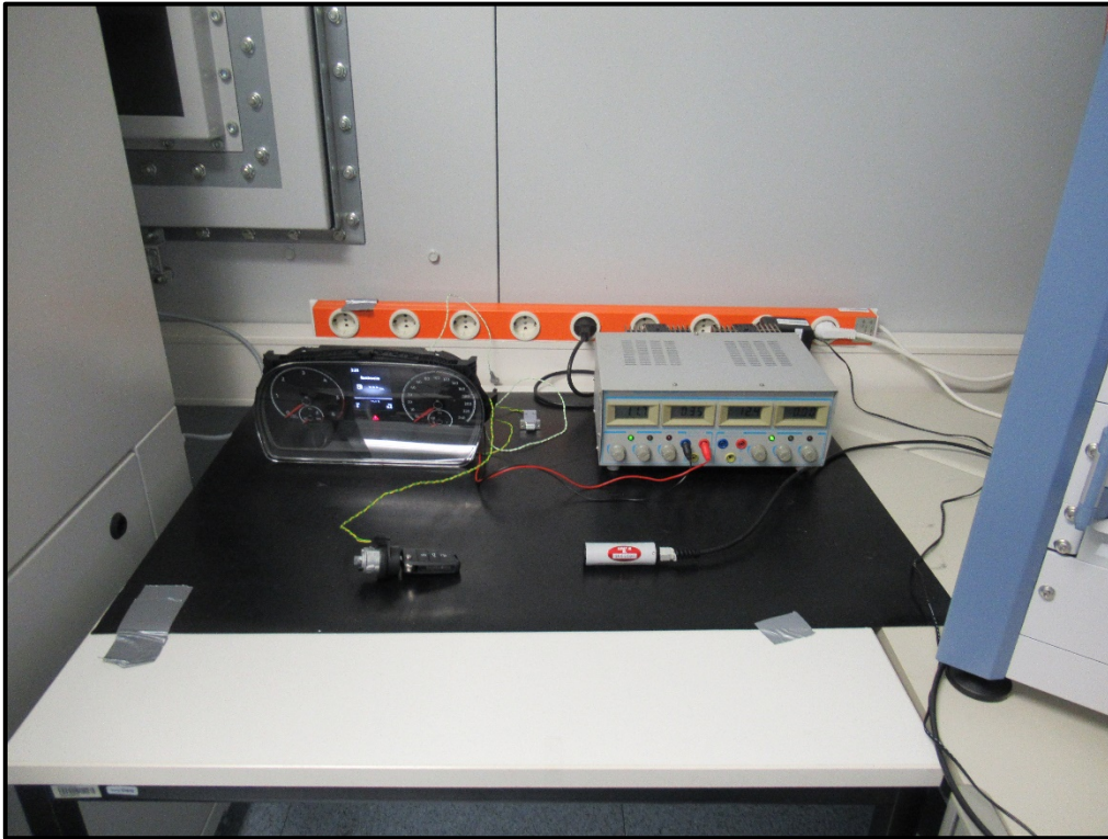
Photo 5: Conducted Bandwidth Measurements
