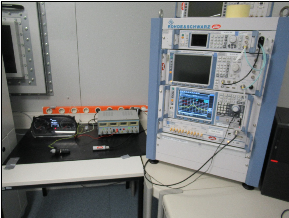
Photo 6: Conducted Bandwidth Measurements
