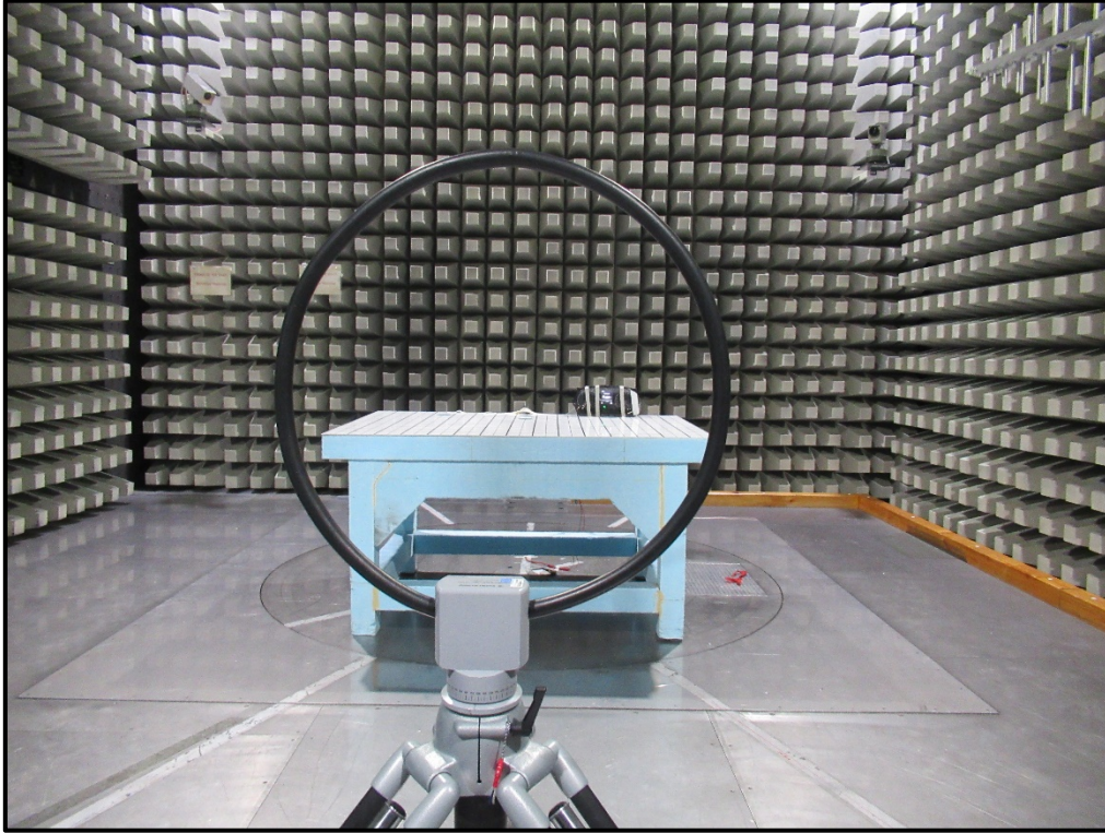
Photo 1: Radiated Fundamental Field Strength & Spurious Emissions – 9 kHz to 30 MHz
