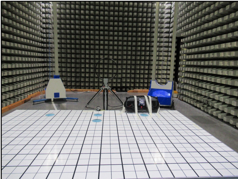
Photo 2: Radiated Fundamental Field Strength & Spurious Emissions – 9 kHz to 30 MHz
