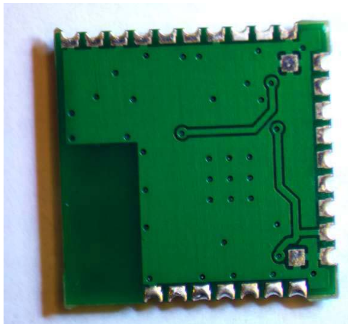
PCB view side 2
