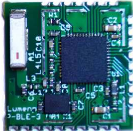
PCB view side 1
