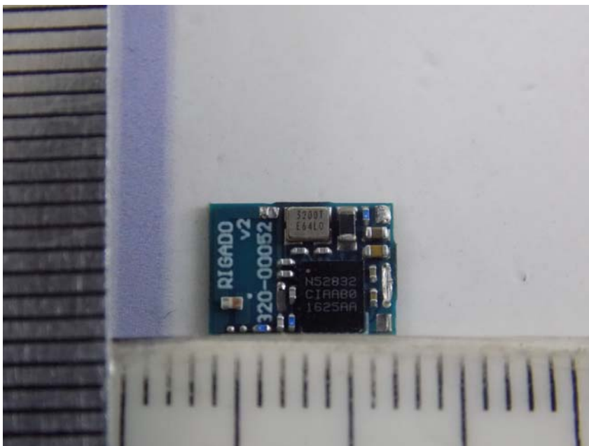
Oscillator view
