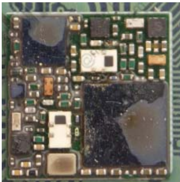
Shielding off view
