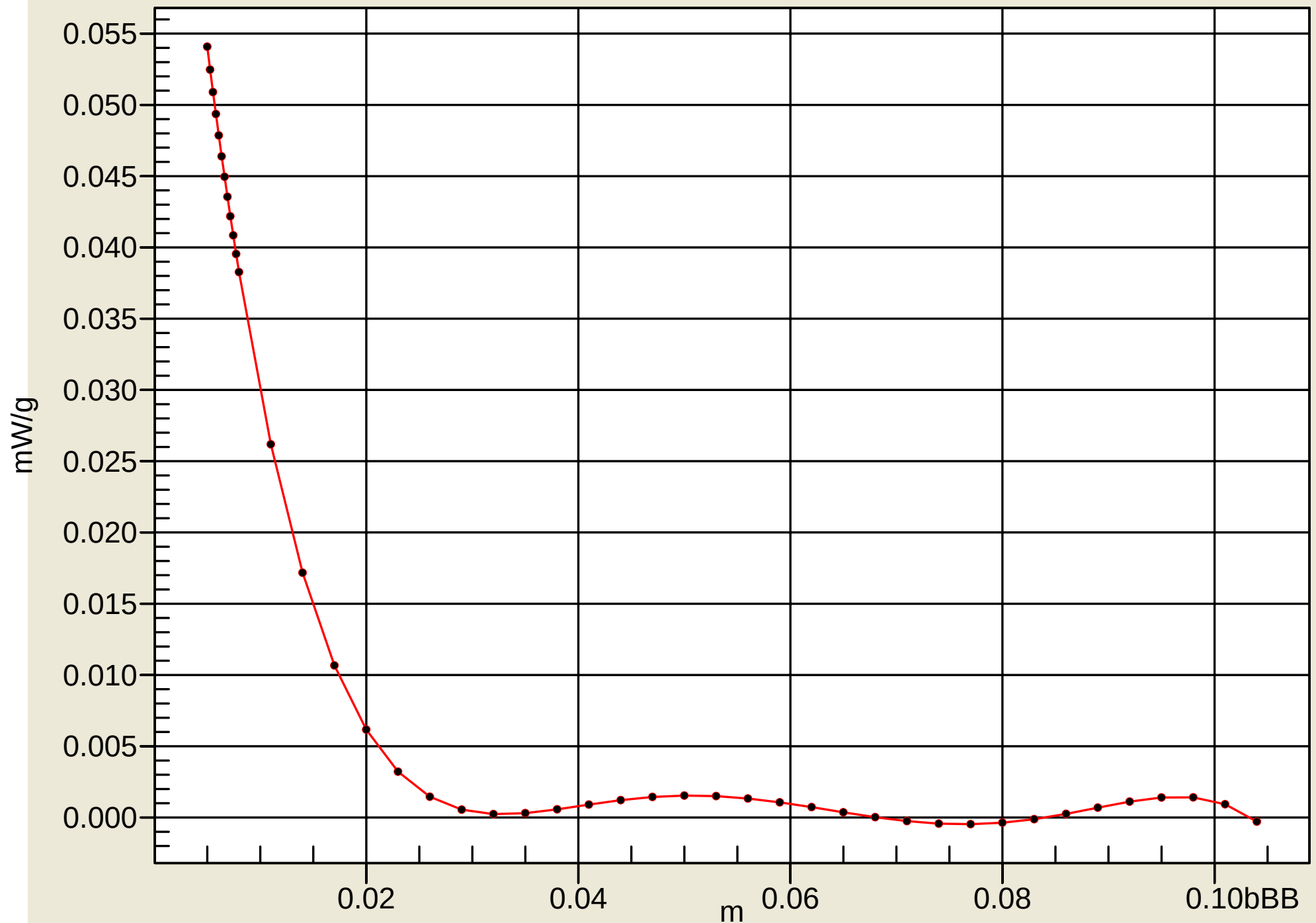
B-Mode Mid Channel SAR; Z Scan: Value Along Z, X=0, Y=0
