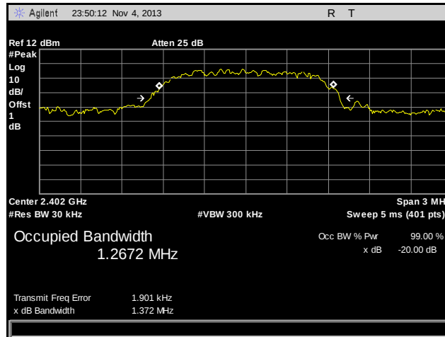
Plot 31. 20 dB Occupied Bandwidth, Low Channel, Pi by 4 DQPDK
