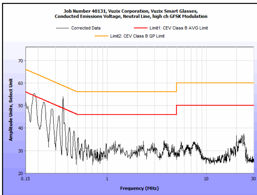
Plot 20. Conducted Emissions, 15.207(a), Neutral, High Channel, GFSK Modulation
