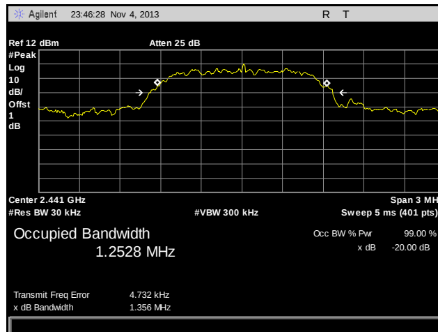
Plot 32. 20 dB Occupied Bandwidth, Mid Channel, Pi by 4 DQPDK
