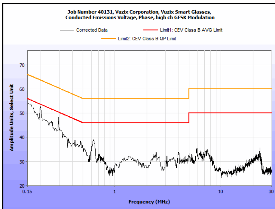
Plot 8. Conducted Emissions, 15.207(a), Phase, High Channel, GFSK Modulation
