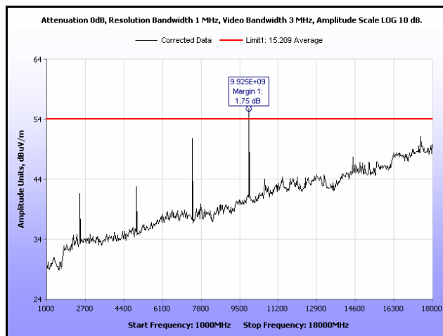
Plot 87. Radiated Spurious Emissions, High Channel, 8DPSK, 1 GHz – 18 GHz
