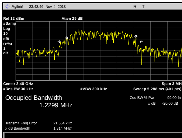
Plot 42. 99% Occupied Bandwidth, High Channel, Pi by 4 DQPDK
