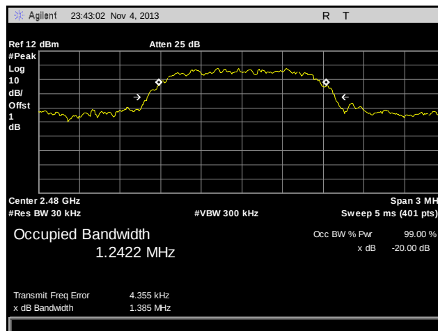
Plot 33. 20 dB Occupied Bandwidth, High Channel, Pi by 4 DQPDK
