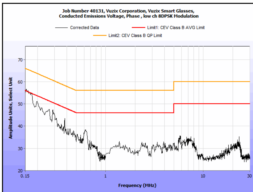
Plot 2. Conducted Emissions, 15.207(a), Phase, Low Channel, 8DPSK Modulation
