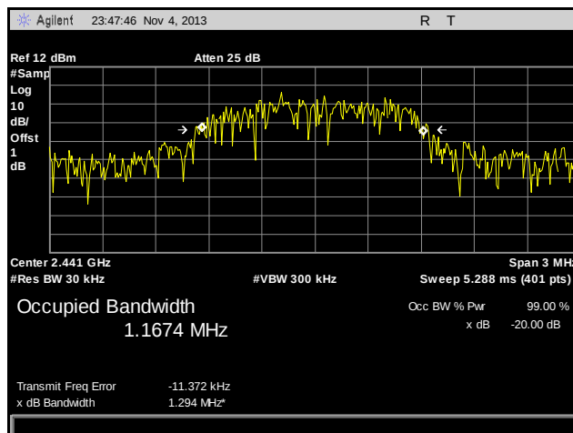
Plot 41. 99% Occupied Bandwidth, Mid Channel, Pi by 4 DQPDK
