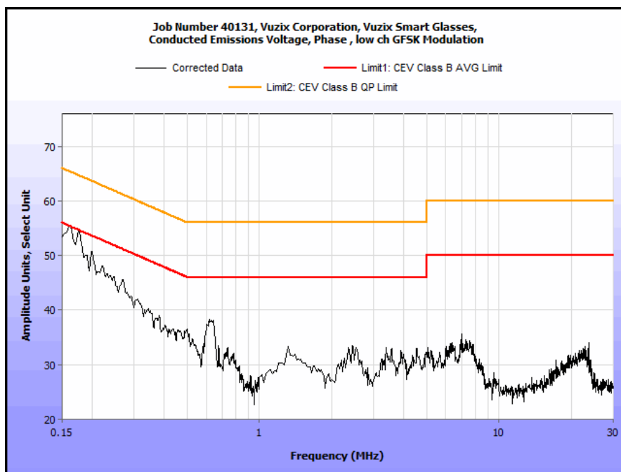
Plot 6. Conducted Emissions, 15.207(a), Phase Low Channel, GFSK Modulation
