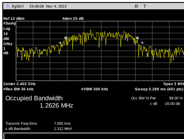
Plot 40. 99% Occupied Bandwidth, Low Channel, Pi by 4 DQPDK
