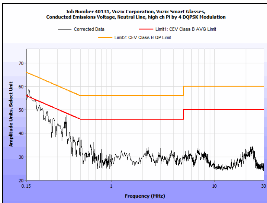
Plot 24. Conducted Emissions, 15.207(a), Neutral, High Channel, Pi by 4 DQPSK Modulation
