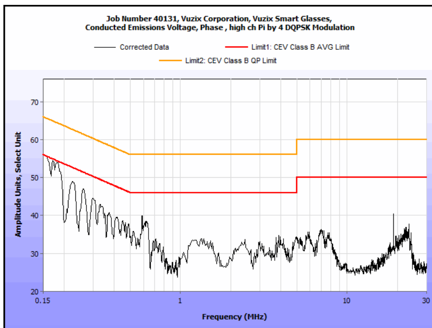
Plot 12. Conducted Emissions, 15.207(a), Phase, High Channel, Pi by 4 DQPSK Modulation
