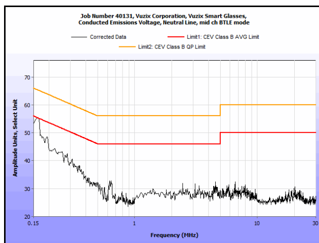
Plot 5. Conducted Emissions, 15.207(a), Neutral Line, Mid Channel
