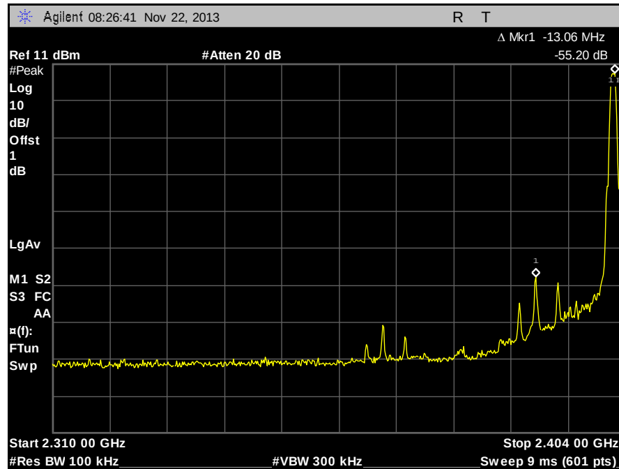
Plot 31. Conducted Band Edge, Low Channel
