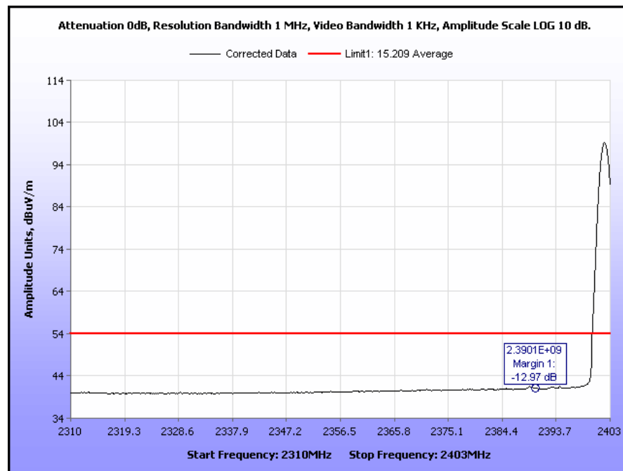
Plot 24. Radiated Restricted Band Edge, Low Channel, Average
