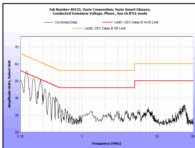
Plot 1. Conducted Emissions, 15.207(a), Phase Line, Low Channel
