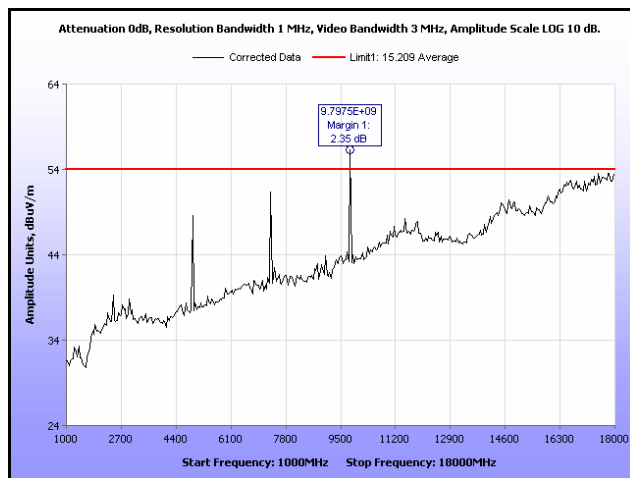
Plot 19. Radiated Spurious Emissions, Mid Channel, 1 GHz – 18 GHz
