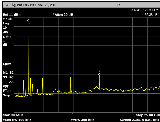
Plot 28. Conducted Spurious Emissions, Low Channel
