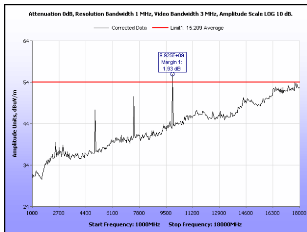
Plot 22. Radiated Spurious Emissions, High Channel, 1 GHz – 18 GHz
