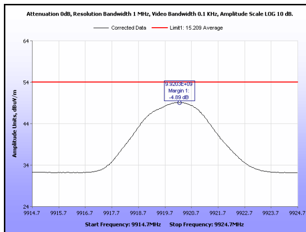
Plot 23. Radiated Spurious Emissions, High Channel, 1 GHz – 18 GHz, 9.92 GHz
