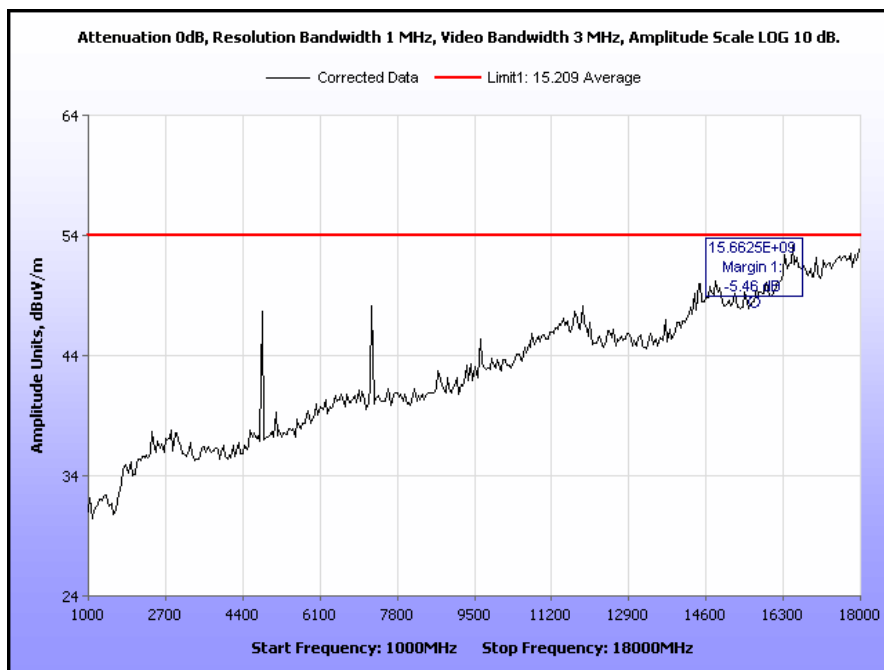
Plot 17. Radiated Spurious Emissions, Low Channel, 1 GHz – 18 GHz
