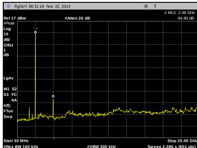
Plot 30. Conducted Spurious Emissions, High Channel
