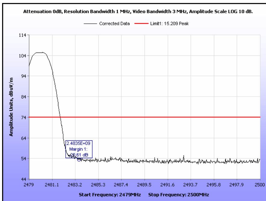
Plot 27. Radiated Restricted Band Edge, High Channel, Peak
