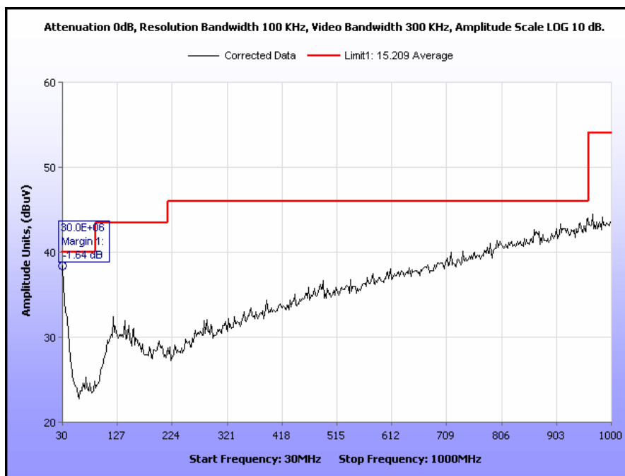
Plot 16. Radiated Spurious Emissions, Low Channel, 30 MHz – 1 GHz
