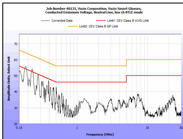
Plot 4. Conducted Emissions, 15.207(a), Neutral Line, Low Channel
