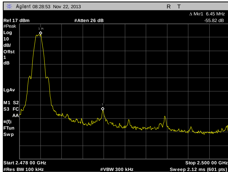
Plot 32. Conducted Band Edge, High Channel
