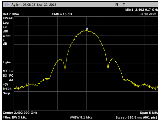
Plot 33. Peak Power Spectral Density, Low Channel
