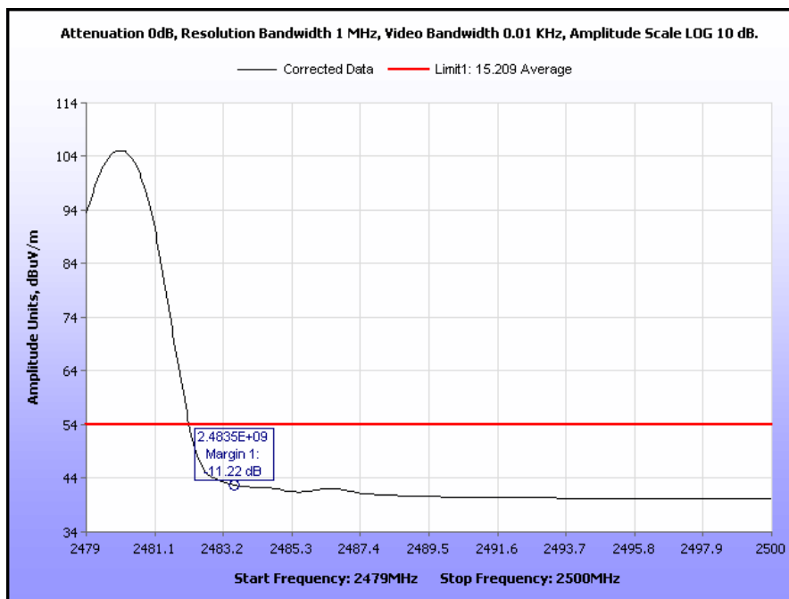
Plot 26. Radiated Restricted Band Edge, High Channel, Average
