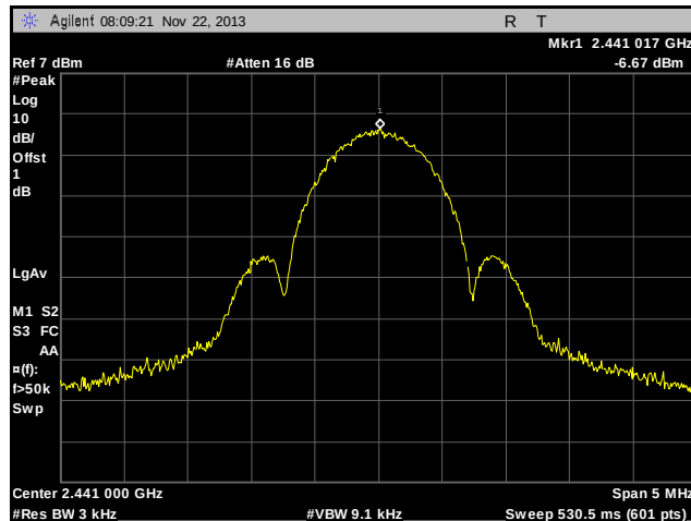
Plot 34. Peak Power Spectral Density, Mid Channel
