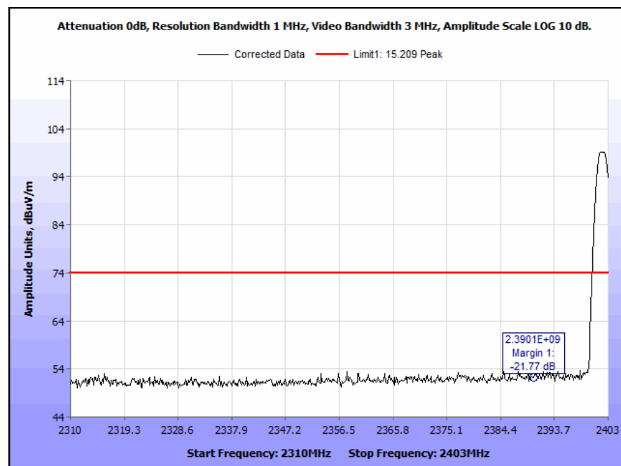
Plot 25. Radiated Restricted Band Edge, Low Channel, Peak
