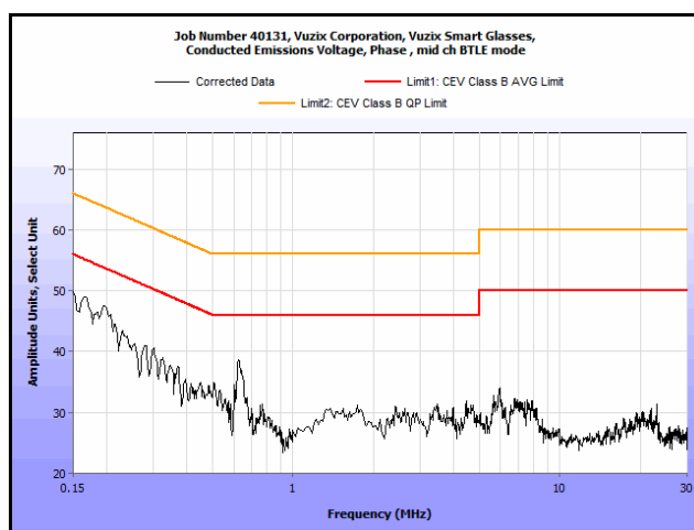
Plot 2. Conducted Emissions, 15.207(a), Phase Line, Mid Channel
