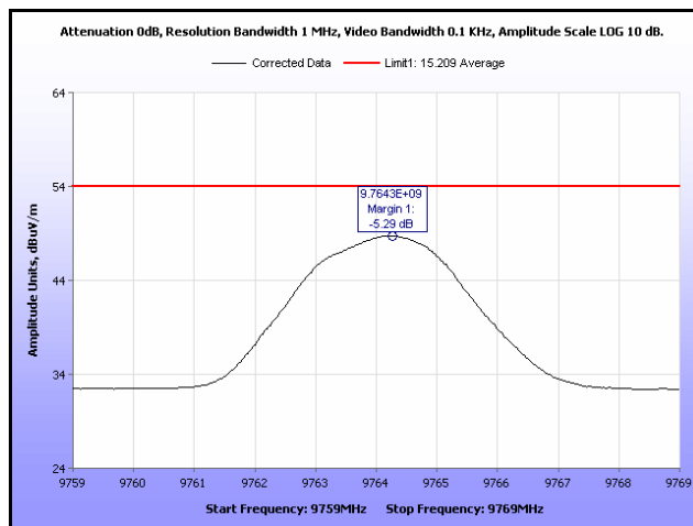
Plot 20. Radiated Spurious Emissions, Mid Channel, 1 GHz – 18 GHz, 9.764 GHz
