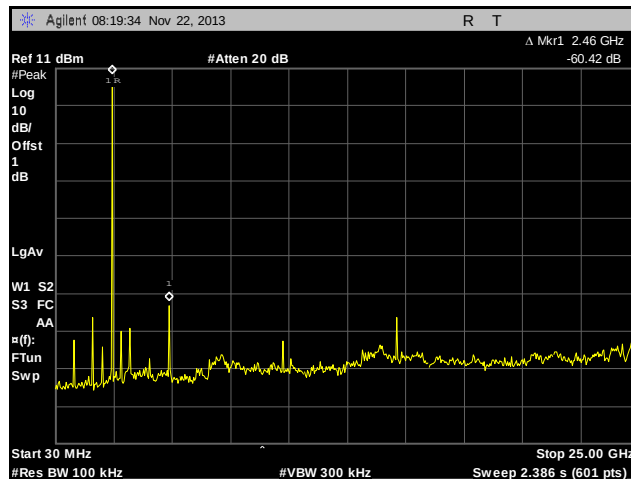
Plot 29. Conducted Spurious Emissions, Mid Channel
