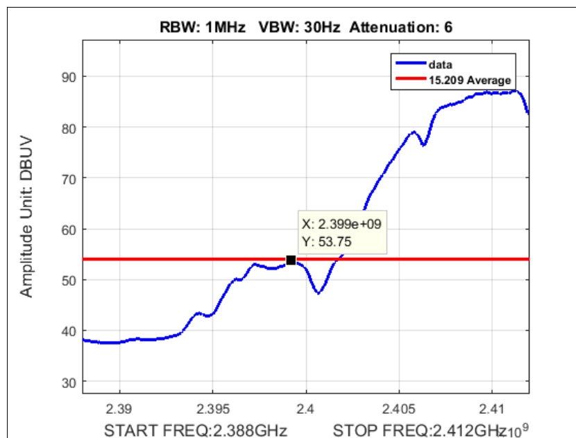
Plot 151. Average Radiated Band Edge, SISO, b mode, port a, Low Channel, 2412M at 19.375 dBm
