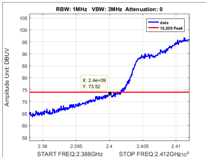
Plot 189. Peak Radiated Band Edge, MIMO, HT8, 40M, Low Channel, 2422M at 19 dBm
