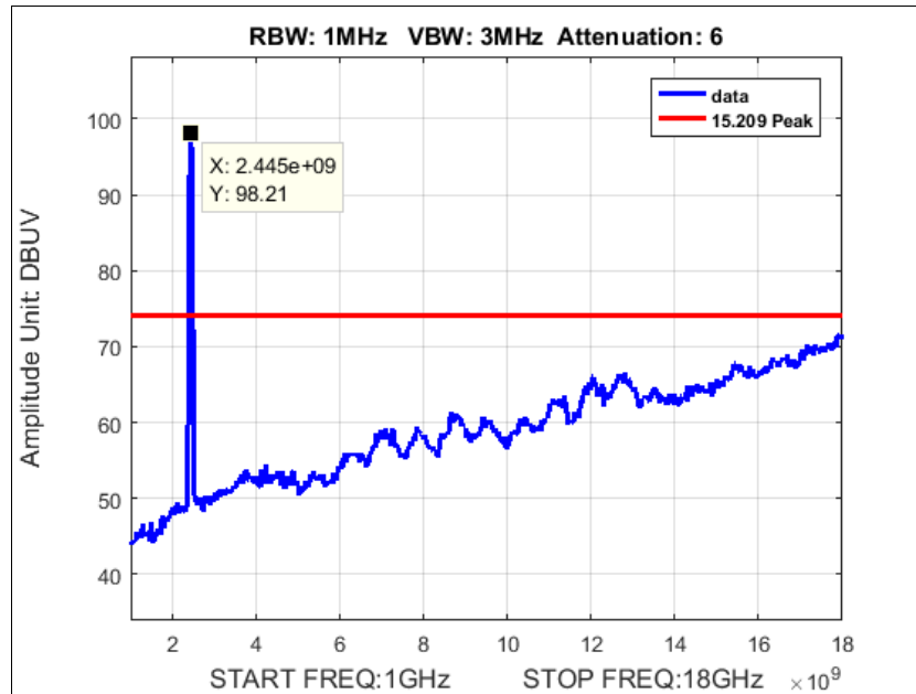
Plot 133. Peak Radiated Spurious Emissions, N40, 40M, Low Channel, 2422, 1-18 GHz
