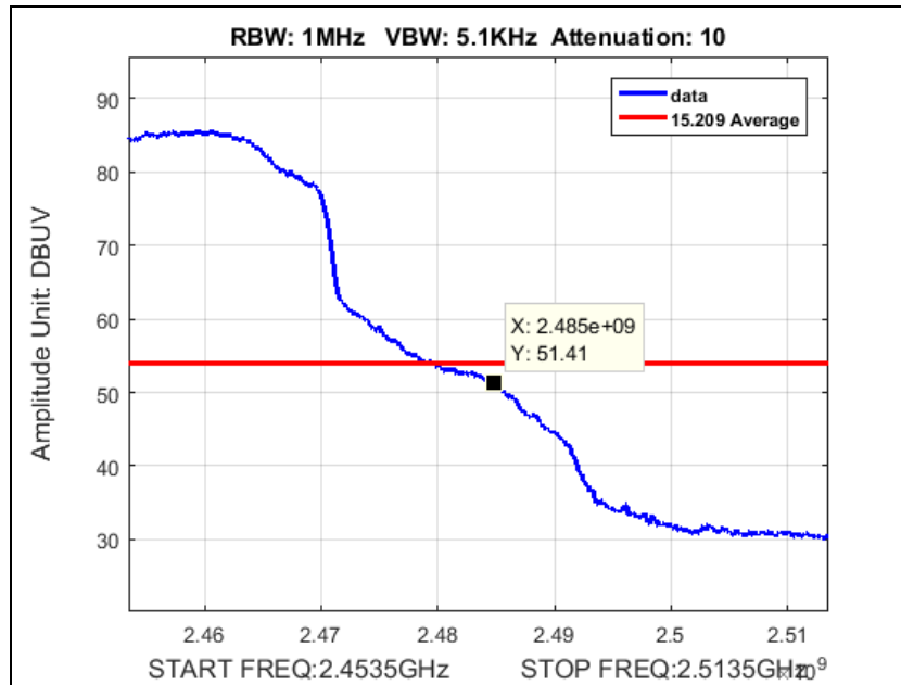
Plot 172. Average Radiated Band Edge, SISO, N40, port b, 2452M at 19 dBm
