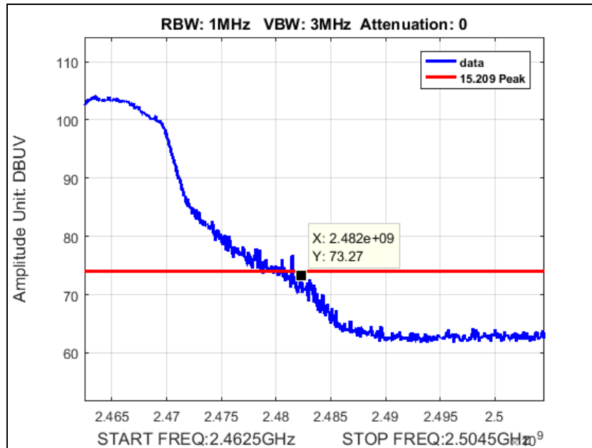
Plot 176. Peak Radiated Band Edge, SISO, g mode, port b, High Channel, 2462M at 19.25 dBm
