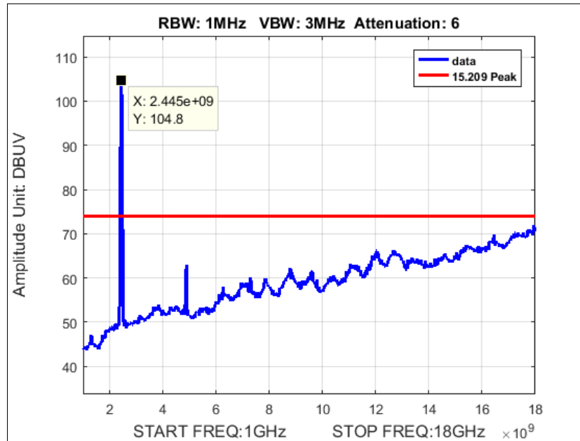
Plot 131. Peak Radiated Spurious Emissions, N20, 20M, Mid Channel, 2437, 1-18 GHz
