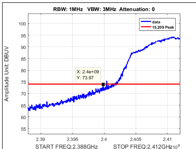
Plot 177. Peak Radiated Band Edge, SISO, g mode, port b, Low Channel, 2412M at 20.25 dBm
