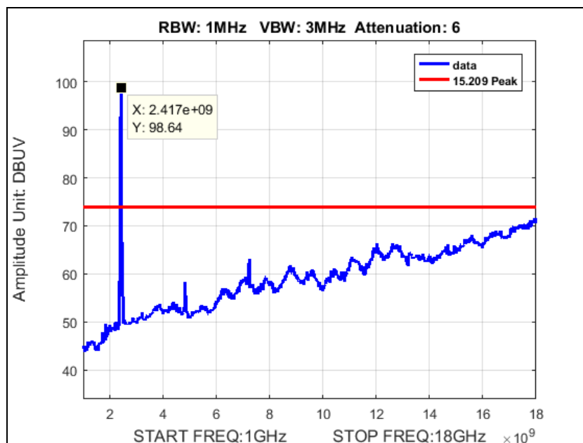
Plot 124. Peak Radiated Spurious Emissions, 20M, b mode, Low Channel, 2412, 1-18 GHz
