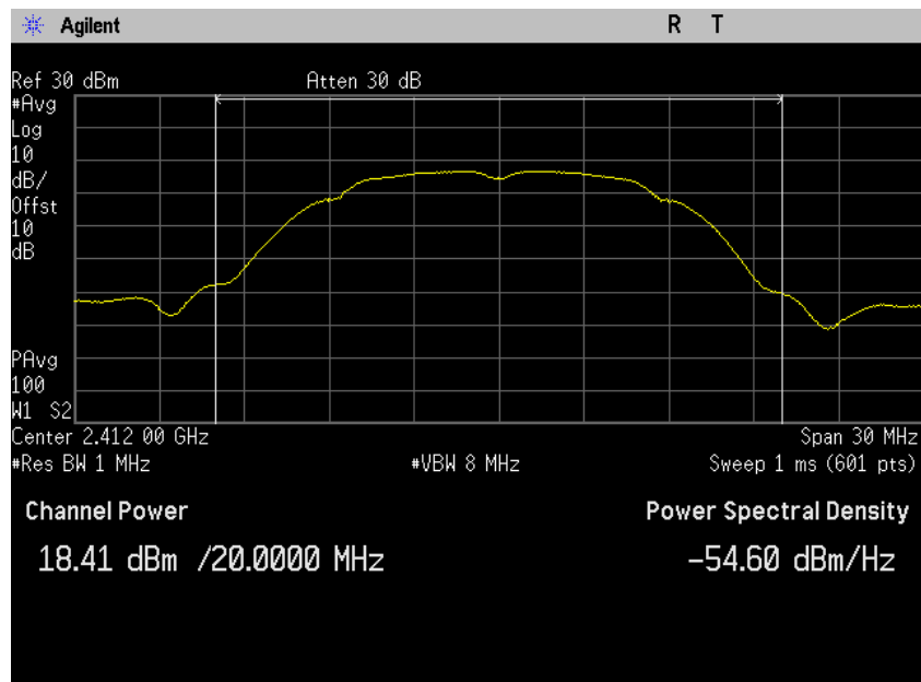
Plot 76. Peak Power Output, SISO, Bandwidth 20M, Ch. 2412M, b mode, port b
