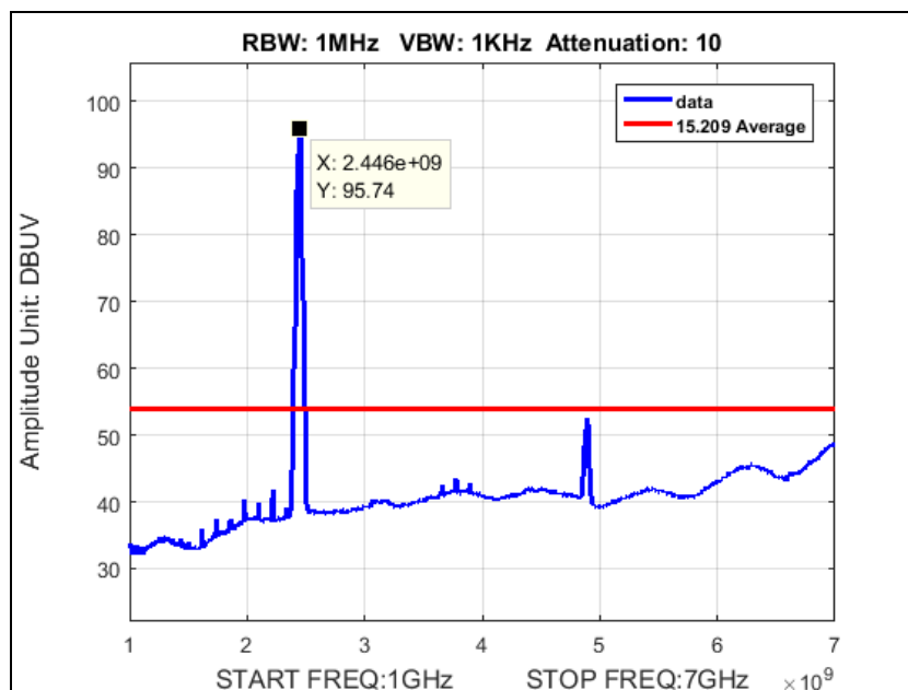
Plot 122. Average Radiated Spurious Emissions, N40, 40M, Mid Channel, 2437, 1-7 GHz
