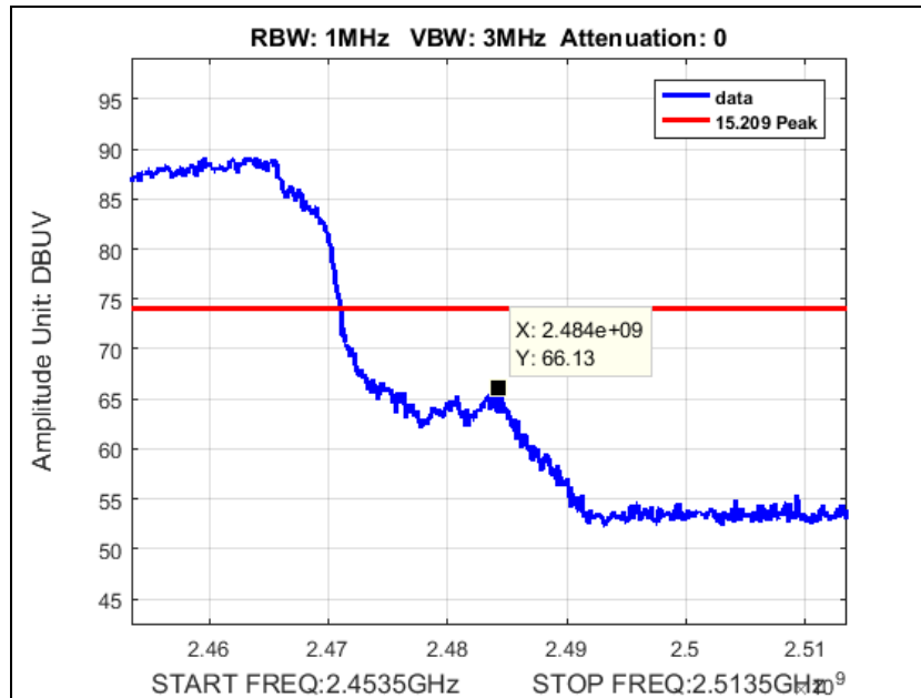
Plot 164. Peak Radiated Band Edge, SISO, N40, port a, 2452M at 20 dBm
