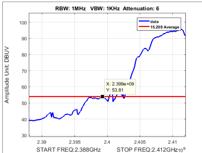
Plot 167. Average Radiated Band Edge, SISO, b mode, port b, Low Channel, 2412M at 18 dBm
