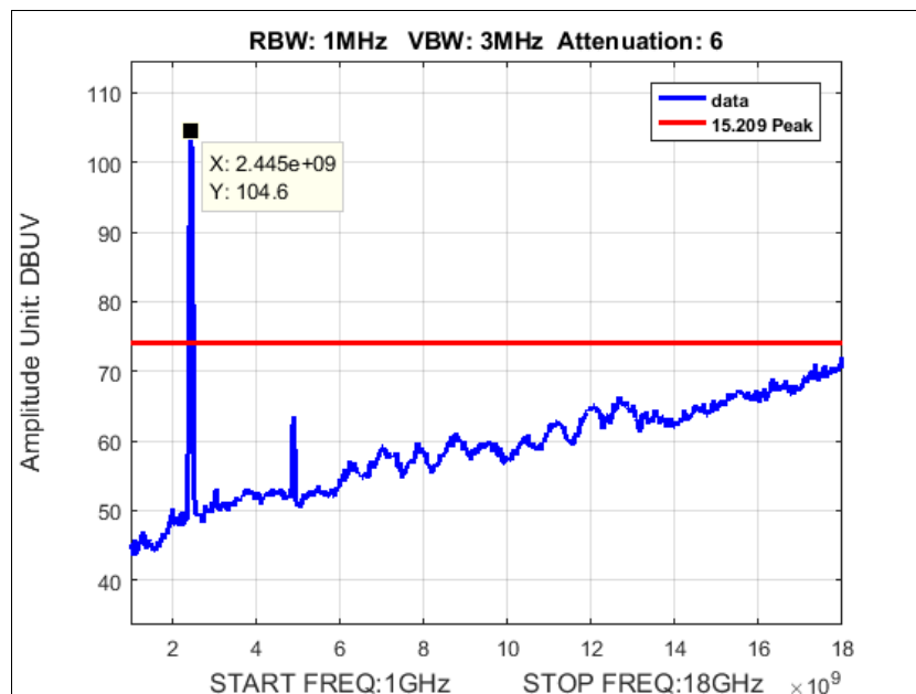
Plot 134. Peak Radiated Spurious Emissions, N40, 40M, Mid Channel, 2437, 1-18 GHz
