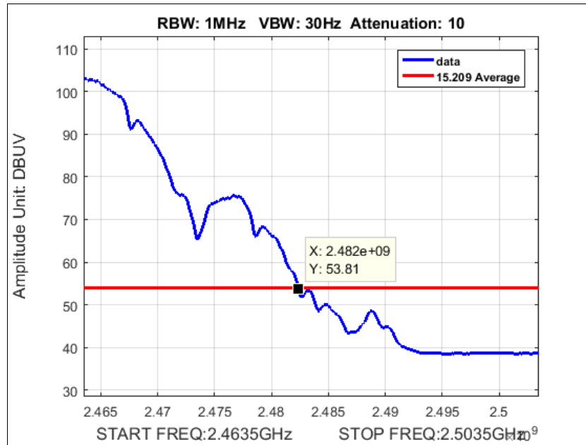
Plot 166. Average Radiated Band Edge, SISO, b mode, port b, 2462M at 22 dBm
