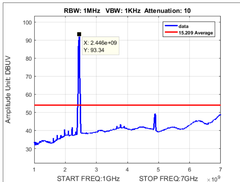
Plot 142. Average Radiated Spurious Emissions, MIMO, HT8, 40M, Mid Channel, 2437, 1-7 GHz
