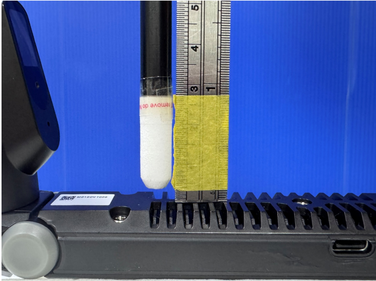
Photo 3: Power Density Front 2_mm
