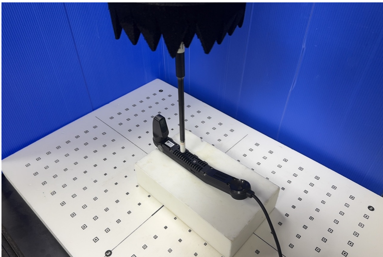
Photo 2: Power Density Front 2_mm
