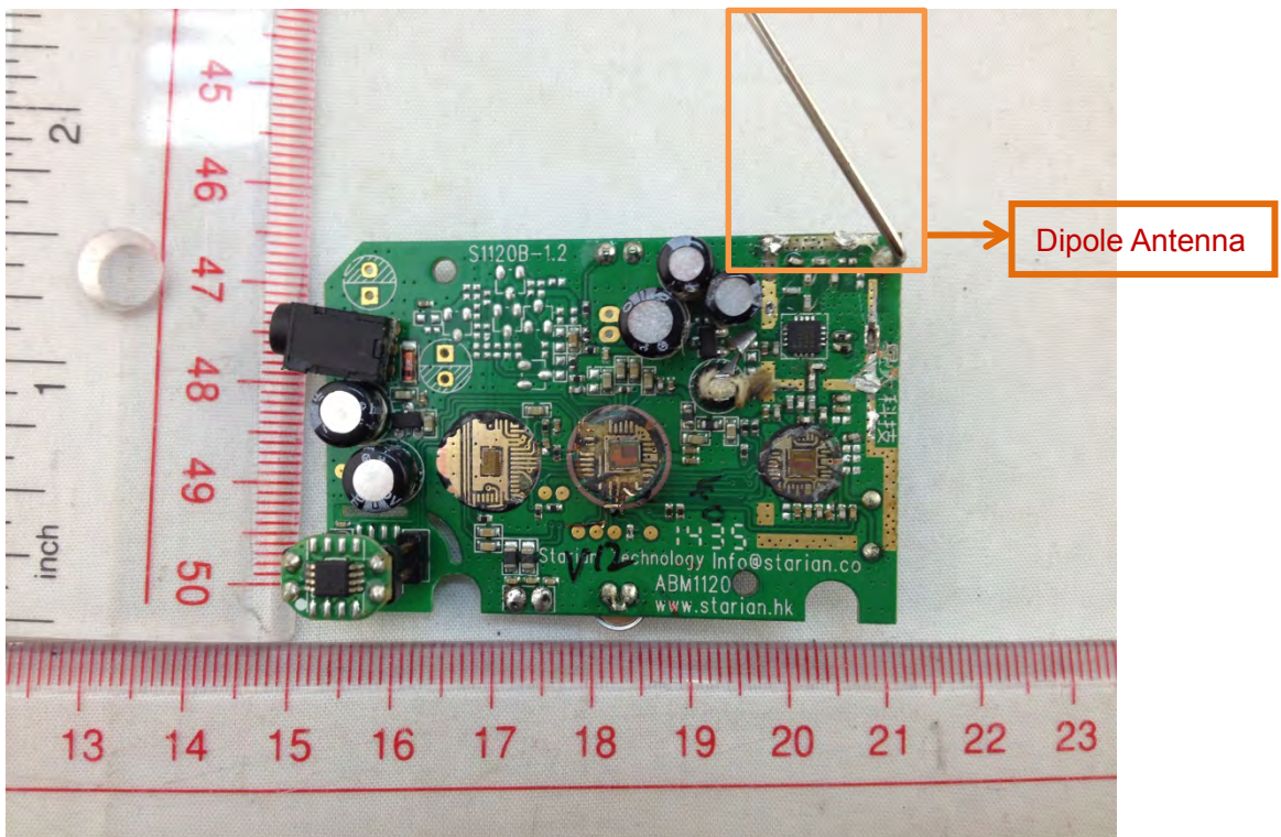
BABY BOARD TOP VIEW 3
