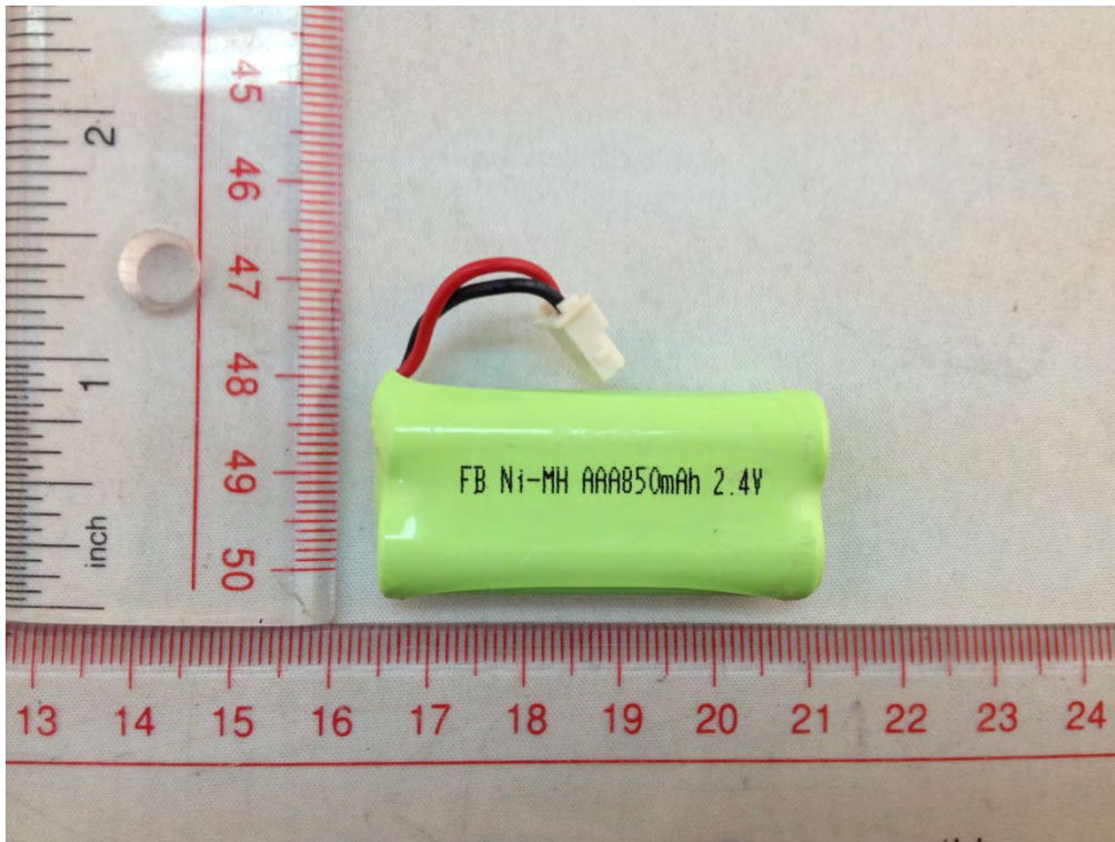
PARENT BATTERY
