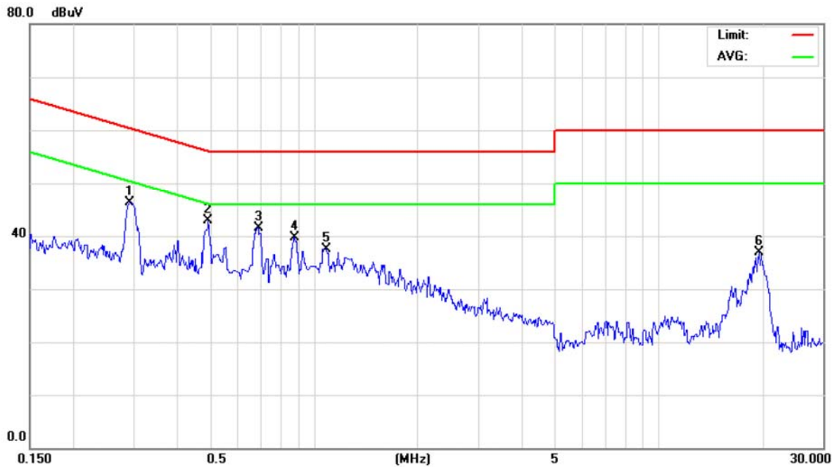
Phase: Line
