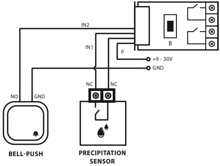
Diagram 5 – example connection to a precipitation sensor
