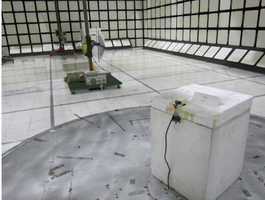
RADIATED PHOTO (BELOW 1 GHz) 3m – Dimmer2 and Bypass2
