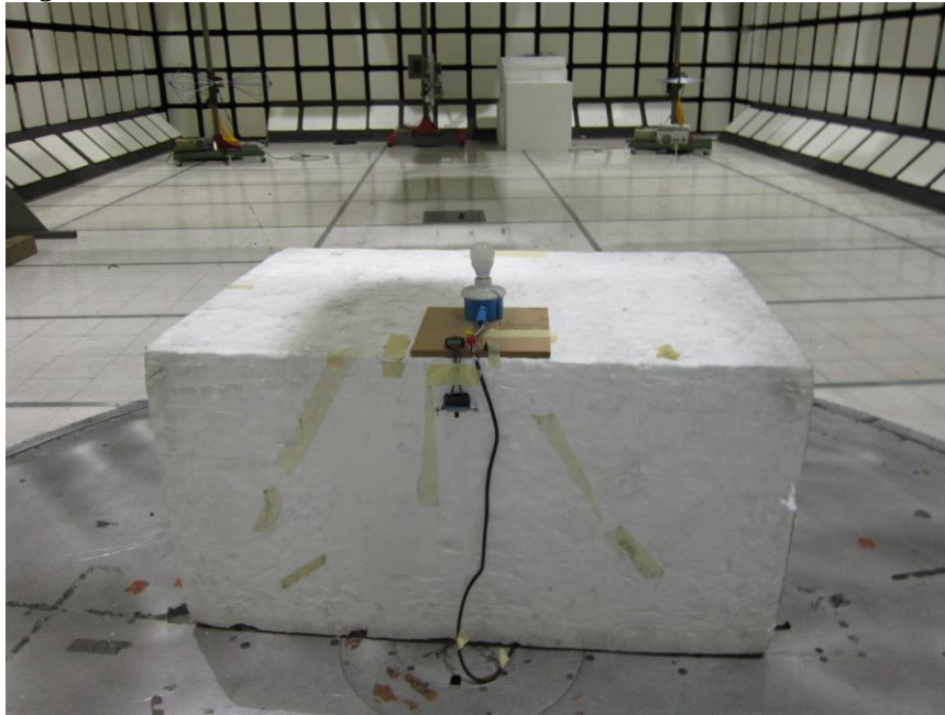
RADIATED PHOTO (30MHz to 1 GHz) 10m – Dimmer2 and Bypass2 Digital
