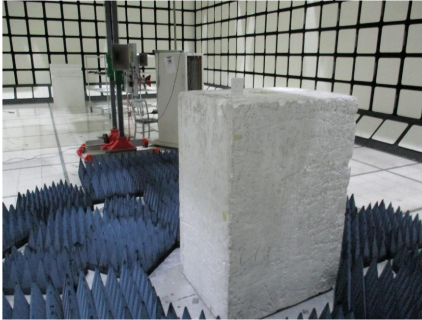
RADIATED PHOTO (ABOVE 1 GHz) Transmitter Setup
