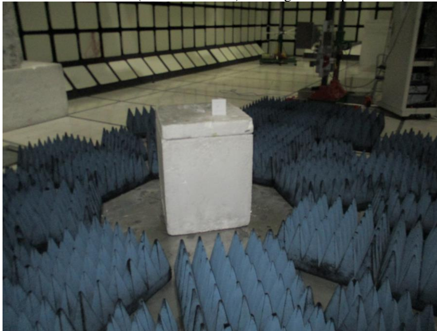
RADIATED PHOTO (ABOVE 1 GHz) RX/Digital Setup
