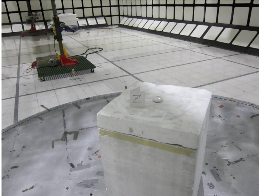
RADIATED PHOTO (BELOW 1 GHz) 3m – Wireless
