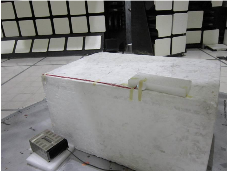
X-AXIS PHOTO – Wireless
