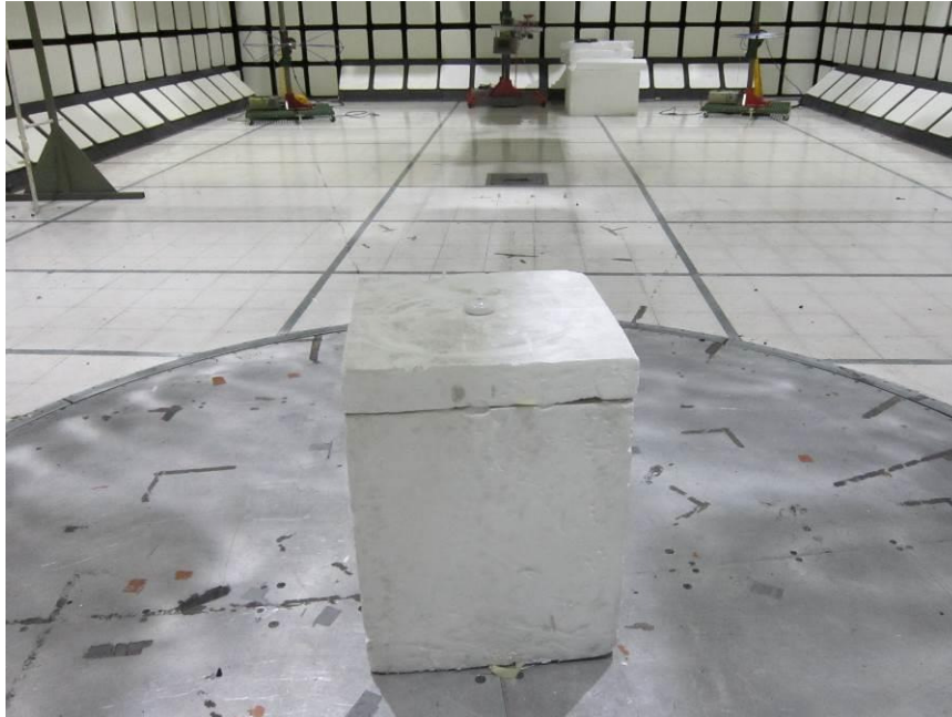
RADIATED PHOTO (BELOW 1 GHz) 10m – Wireless
