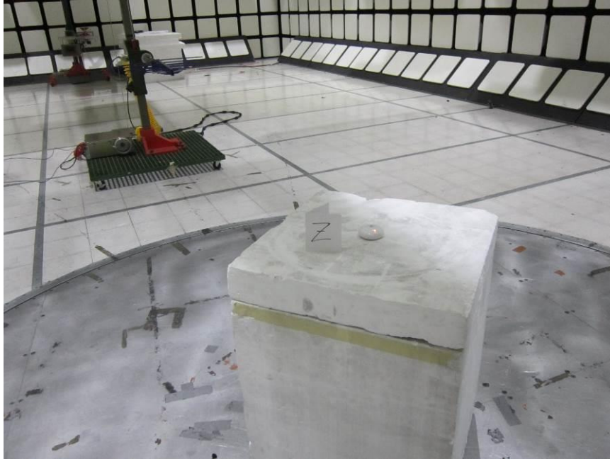
Z-AXIS PHOTO – Wired
