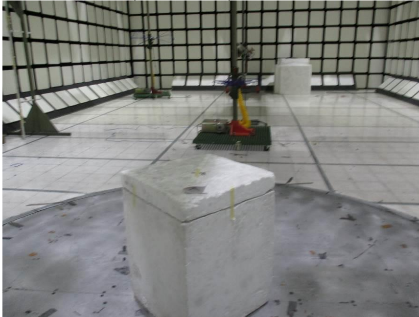
RADIATED PHOTO (BELOW 1 GHz) 3m
