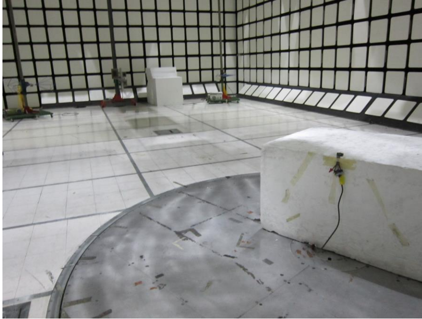
RADIATED PHOTO (30 to 1000MHz) Digital
