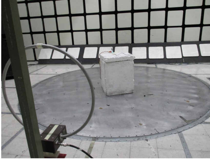
RADIATED PHOTO (9 kHz to 30 MHz) 3m
