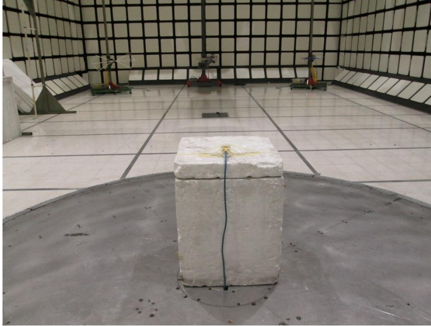
RADIATED PHOTO (BELOW 1 GHz) 10m TX
