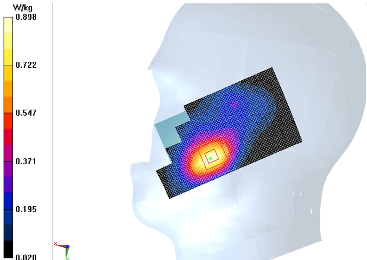
Fig.3 1900 MHz CH810
