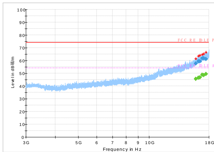
Fig.53 Radiated Spurious Emission (802.11g,Ch11,3GHz~18GHz)
