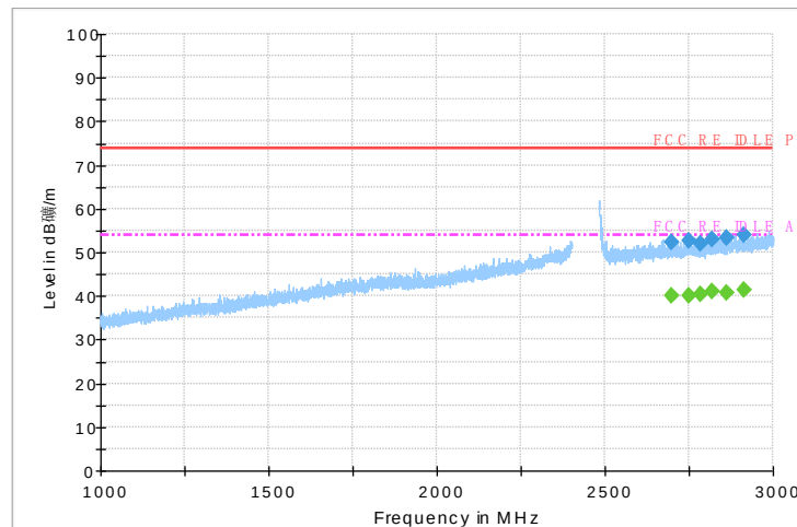
Fig.52 Radiated Spurious Emission (802.11g,Ch11,1GHz~3GHz)
