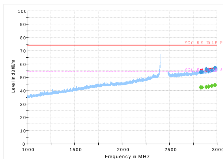
Fig.57 Radiated Spurious Emission (802.11 n-20MHz,Ch1,1GHz~3GHz)
