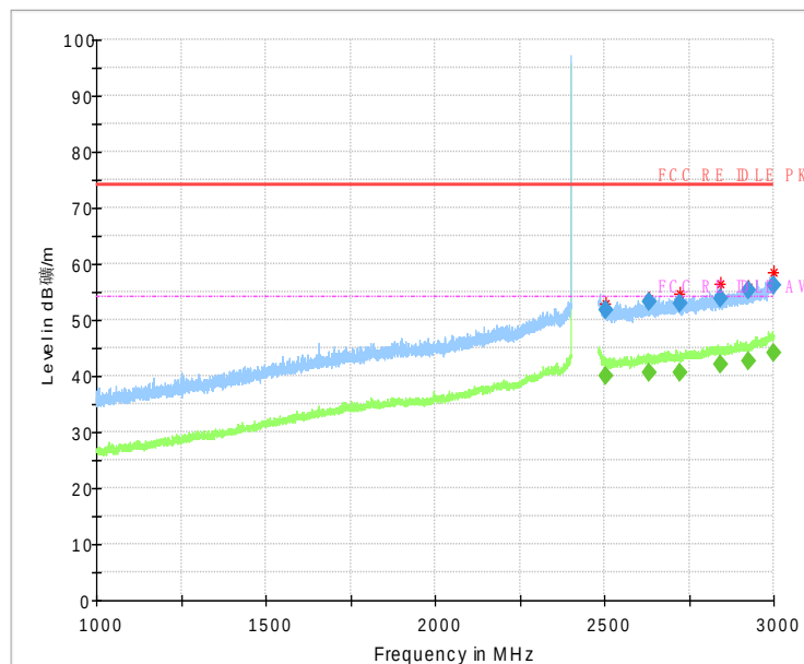
Fig.53 Radiated emission: 8DPSK, Ch0, 1GHz~3GHz
