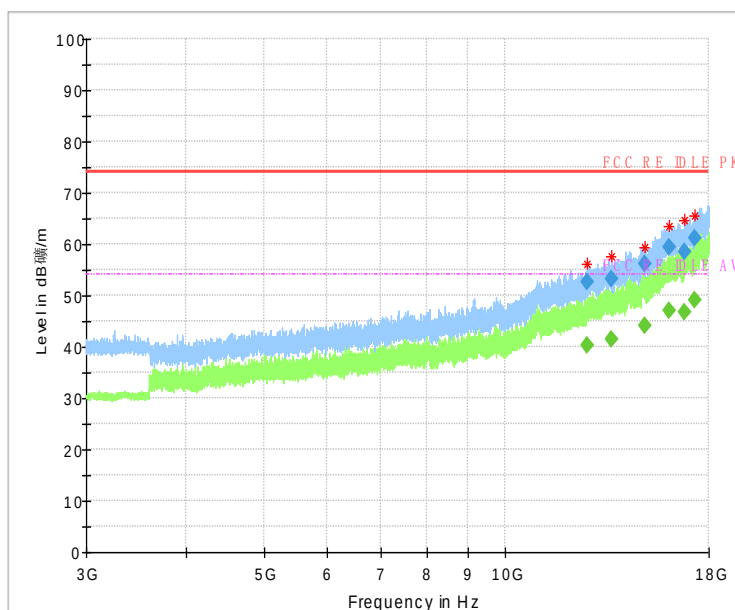
Fig.54 Radiated emission: 8DPSK, Ch0, 3GHz~18GHz
