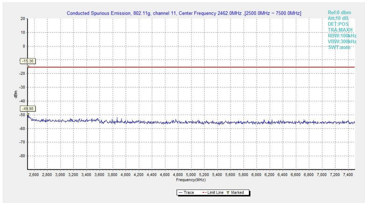
Fig.A.7.1.44 Conducted Spurious Emission (802.11g, Ch11, 2.5 GHz-7.5 GHz)
