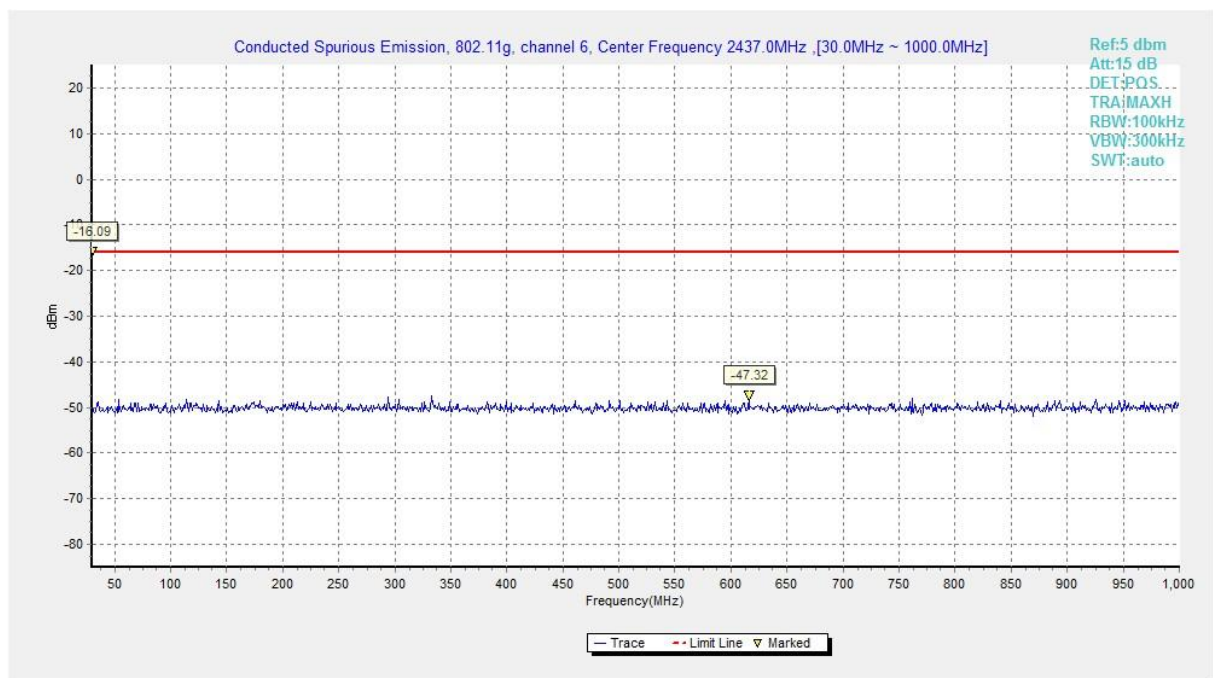
Fig.A.7.1.34 Conducted Spurious Emission (802.11g, Ch6, 30 MHz-1 GHz)
