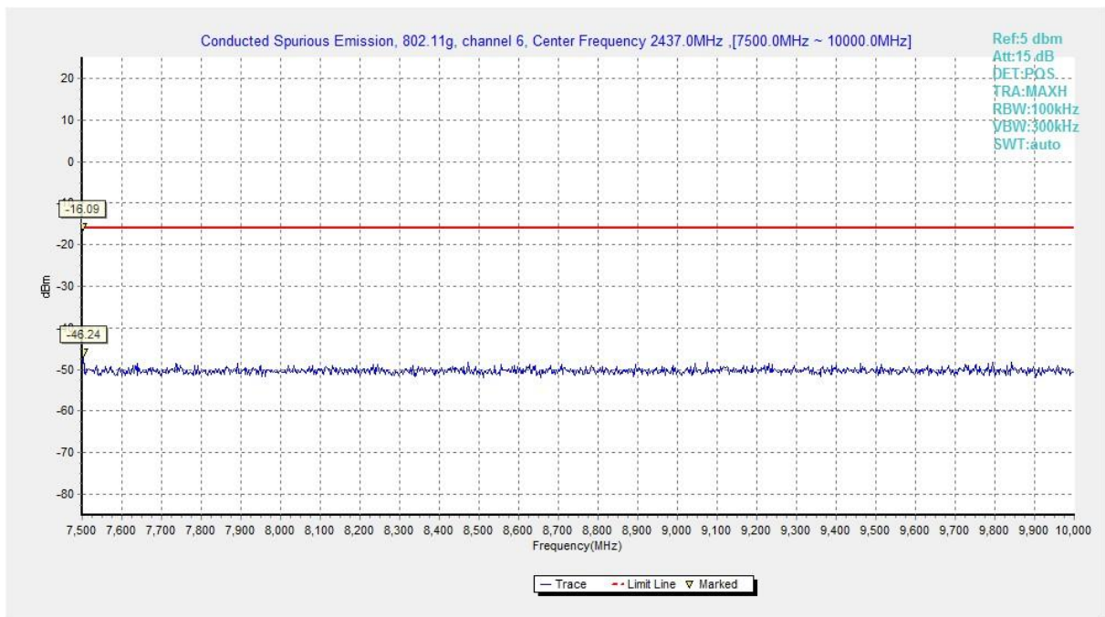
Fig.A.7.1.37 Conducted Spurious Emission (802.11g, Ch6, 7.5 GHz-10 GHz)
