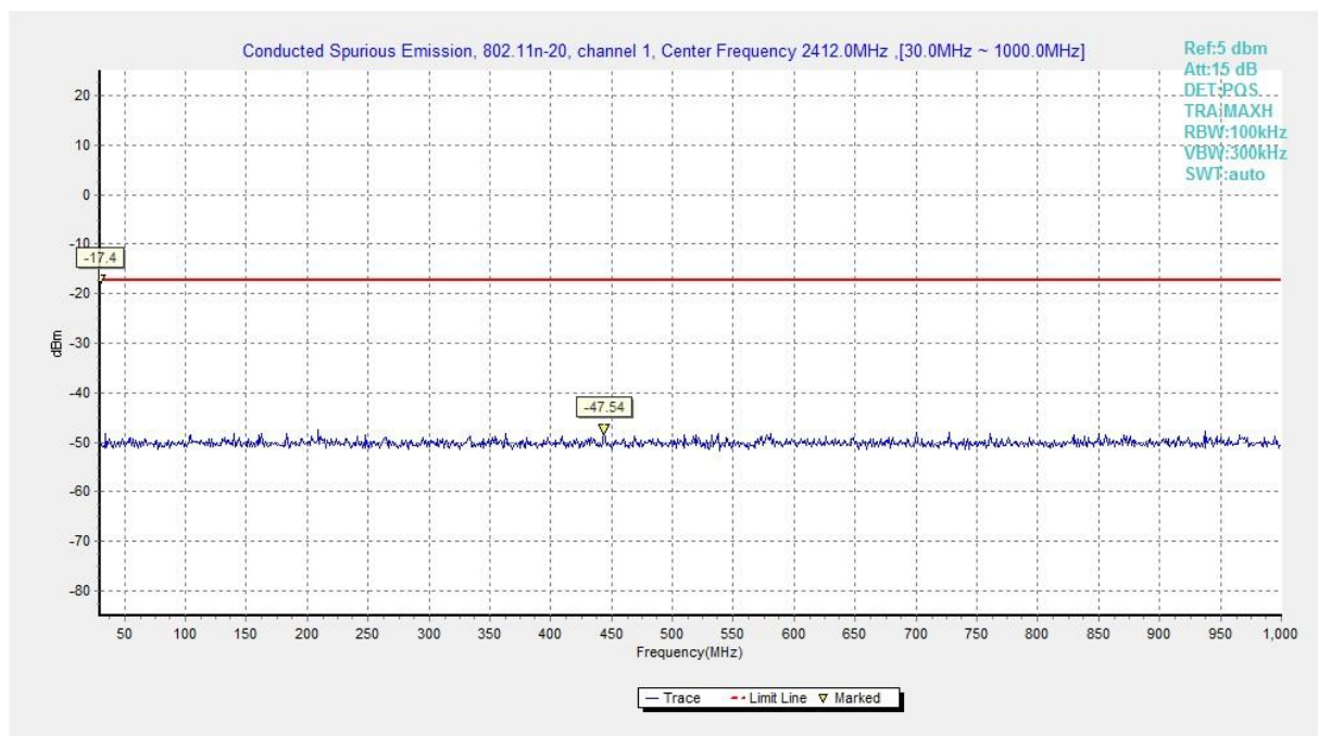
Fig.A.7.1.50 Conducted Spurious Emission (802.11n-HT20, Ch1, 30 MHz-1 GHz)
