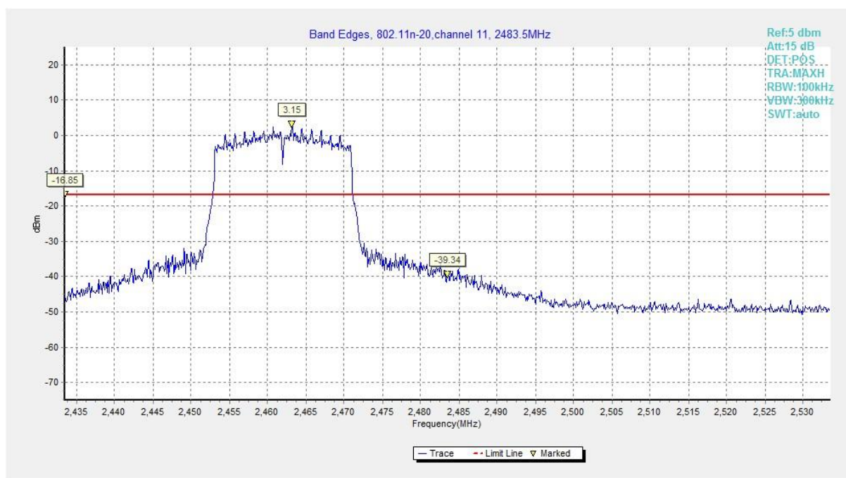
Fig.A.6.6 Band Edges (802.11n-HT20, Ch 11)
