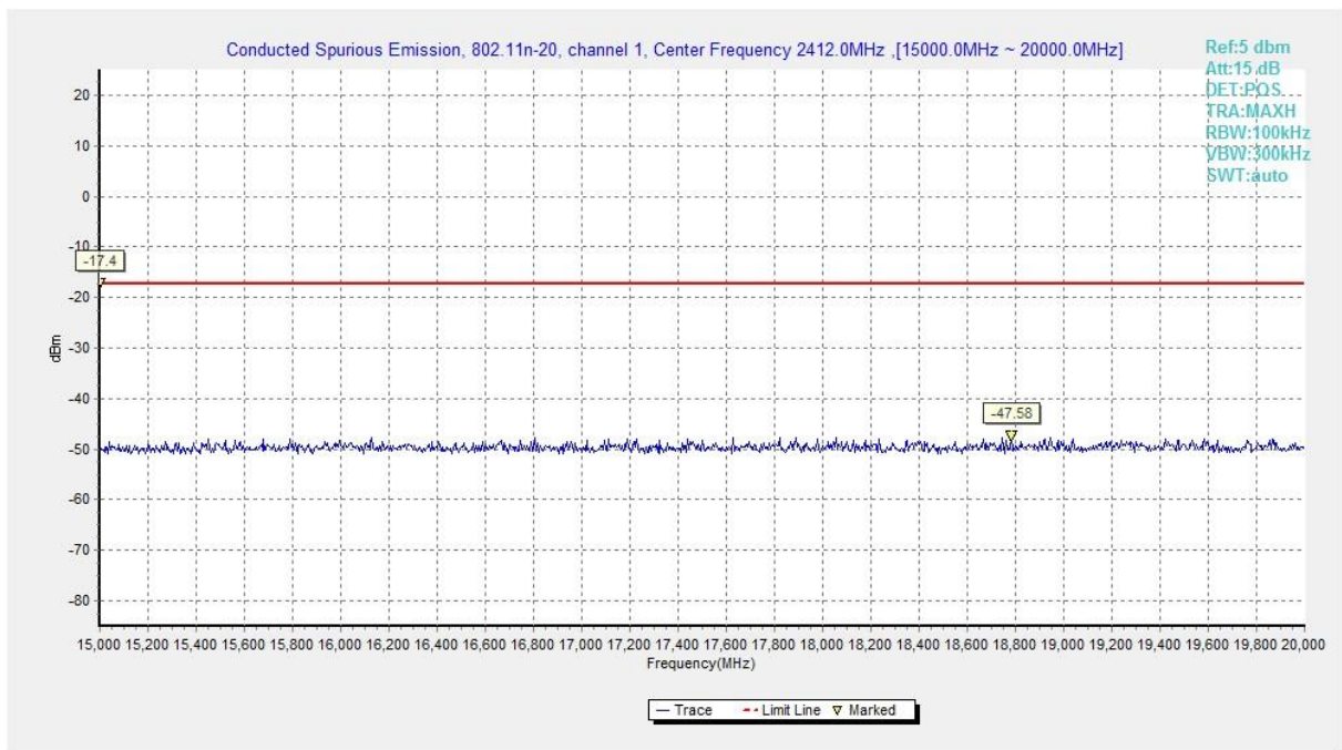
Fig.A.7.1.55 Conducted Spurious Emission (802.11n-HT20, Ch1, 15 GHz-20 GHz)
