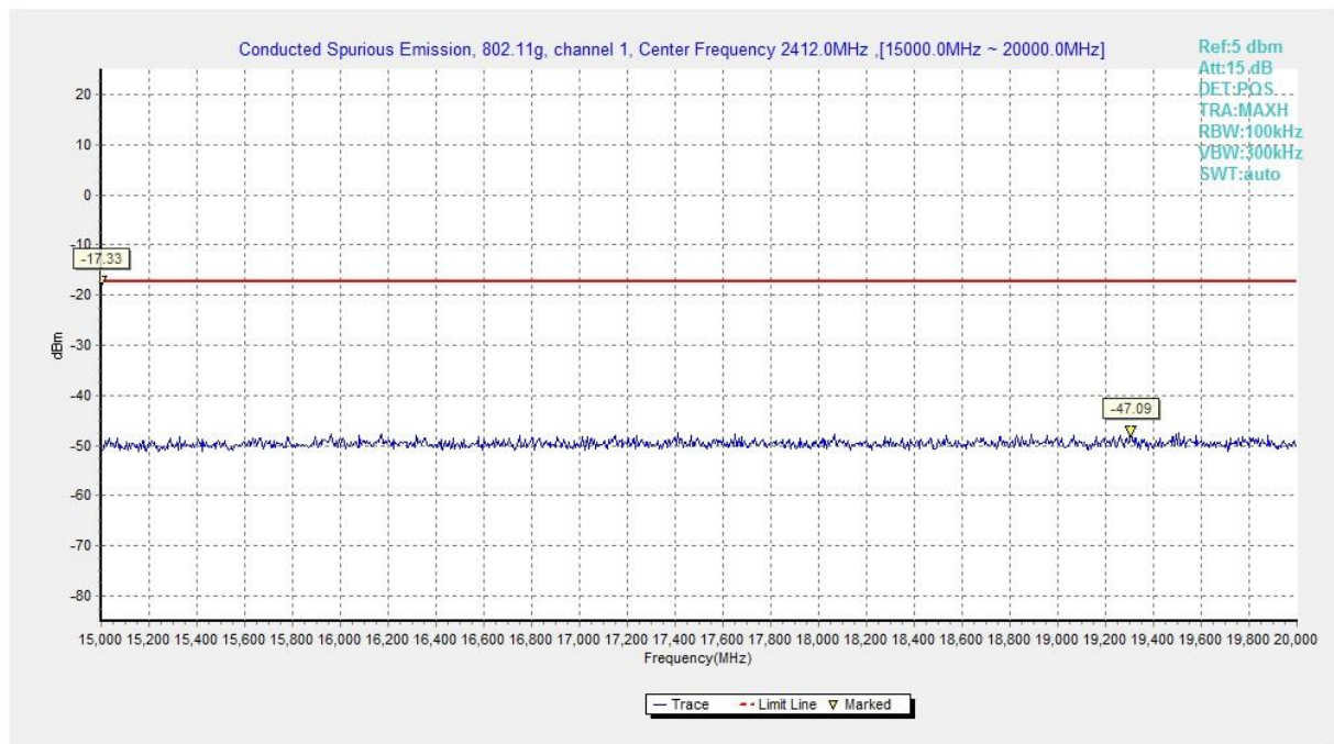
Fig.A.7.1.31 Conducted Spurious Emission (802.11g, Ch1, 15 GHz-20 GHz)
