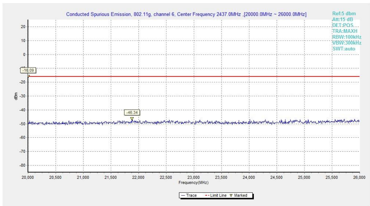
Fig.A.7.1.40 Conducted Spurious Emission (802.11g, Ch6, 20 GHz-26 GHz)
