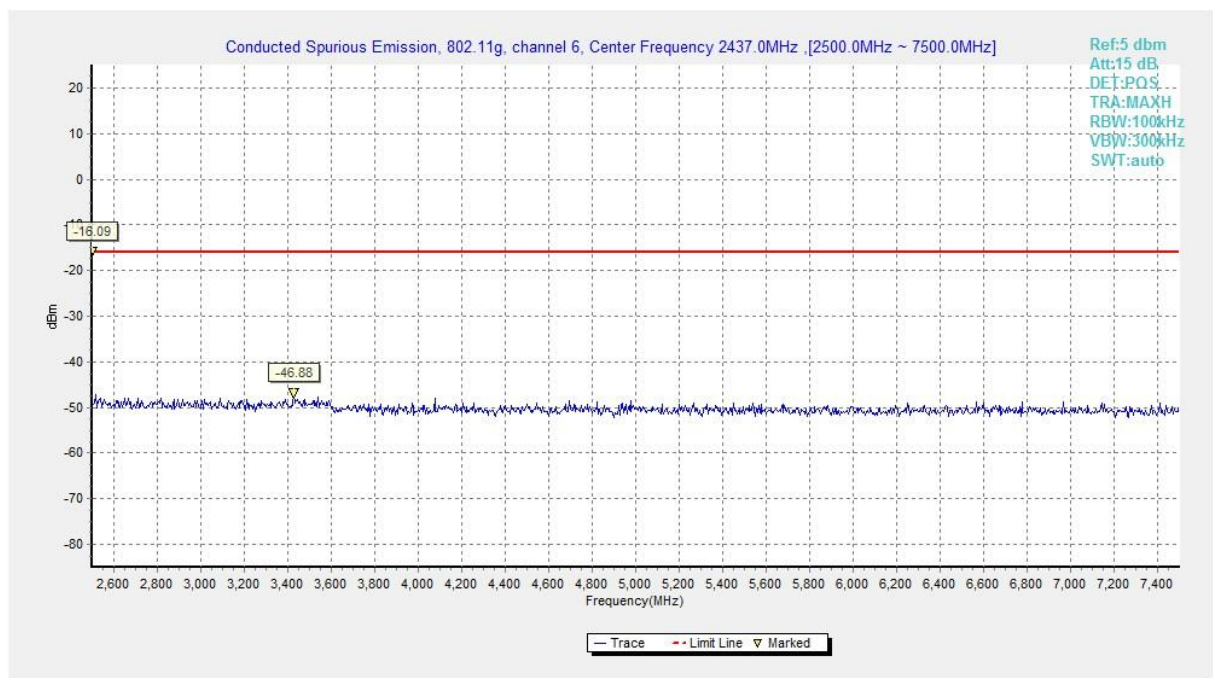
Fig.A.7.1.36 Conducted Spurious Emission (802.11g, Ch6, 2.5 GHz-7.5 GHz)
