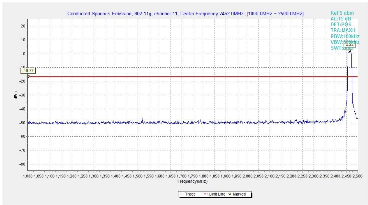
Fig.A.7.1.43 Conducted Spurious Emission (802.11g, Ch11, 1 GHz-2.5 GHz)
