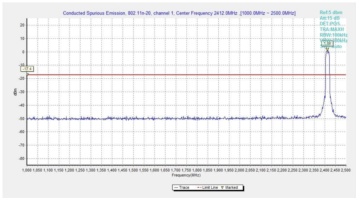
Fig.A.7.1.51 Conducted Spurious Emission (802.11n-HT20, Ch1, 1 GHz-2.5 GHz)
