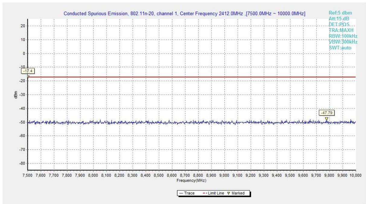
Fig.A.7.1.53 Conducted Spurious Emission (802.11n-HT20, Ch1, 7.5 GHz-10 GHz)
