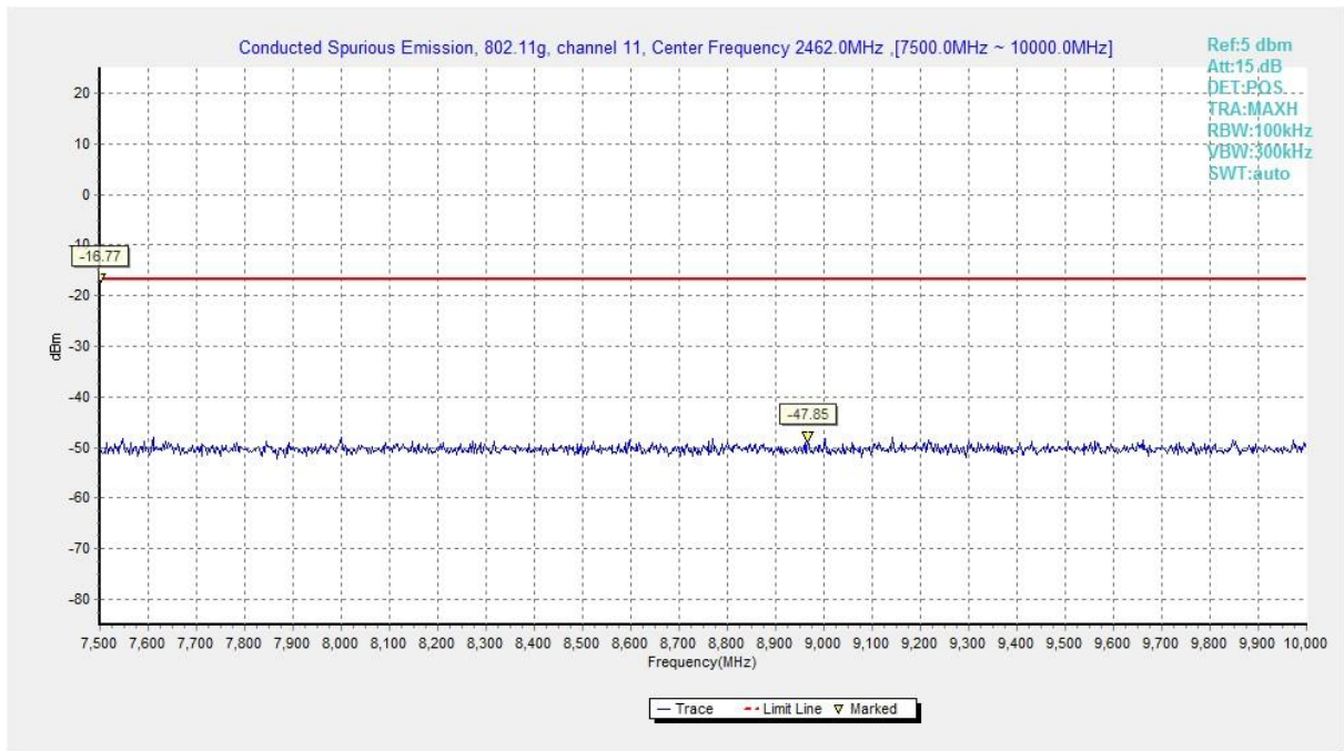
Fig.A.7.1.45 Conducted Spurious Emission (802.11g, Ch11, 7.5 GHz-10 GHz)
