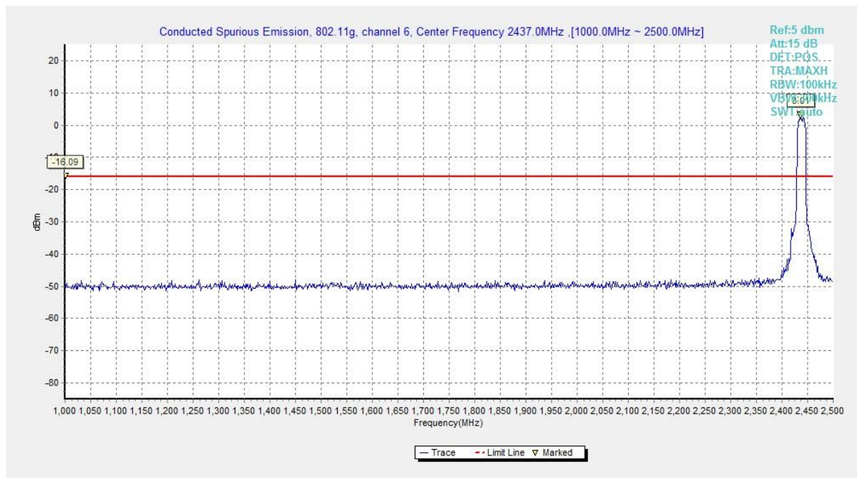
Fig.A.7.1.35 Conducted Spurious Emission (802.11g, Ch6, 1 GHz-2.5 GHz)
