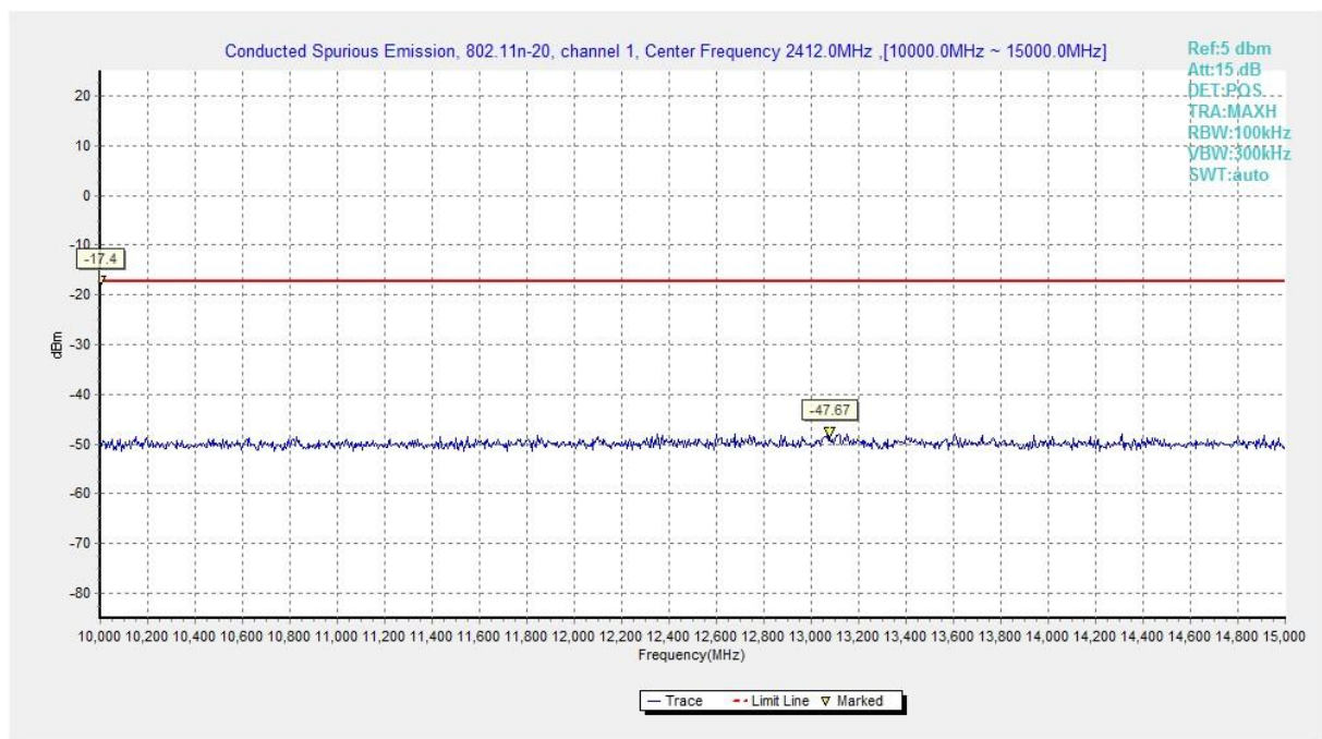
Fig.A.7.1.54 Conducted Spurious Emission (802.11n-HT20, Ch1, 10 GHz-15 GHz)
