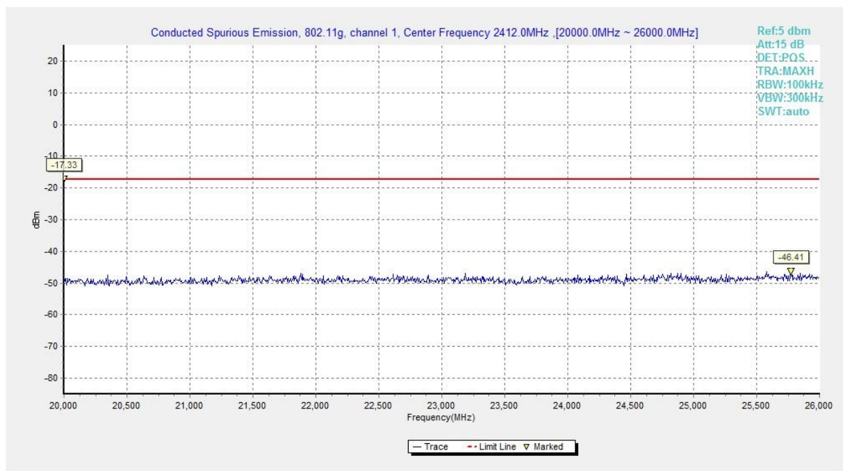
Fig.A.7.1.32 Conducted Spurious Emission (802.11g, Ch1, 20 GHz-26 GHz)
