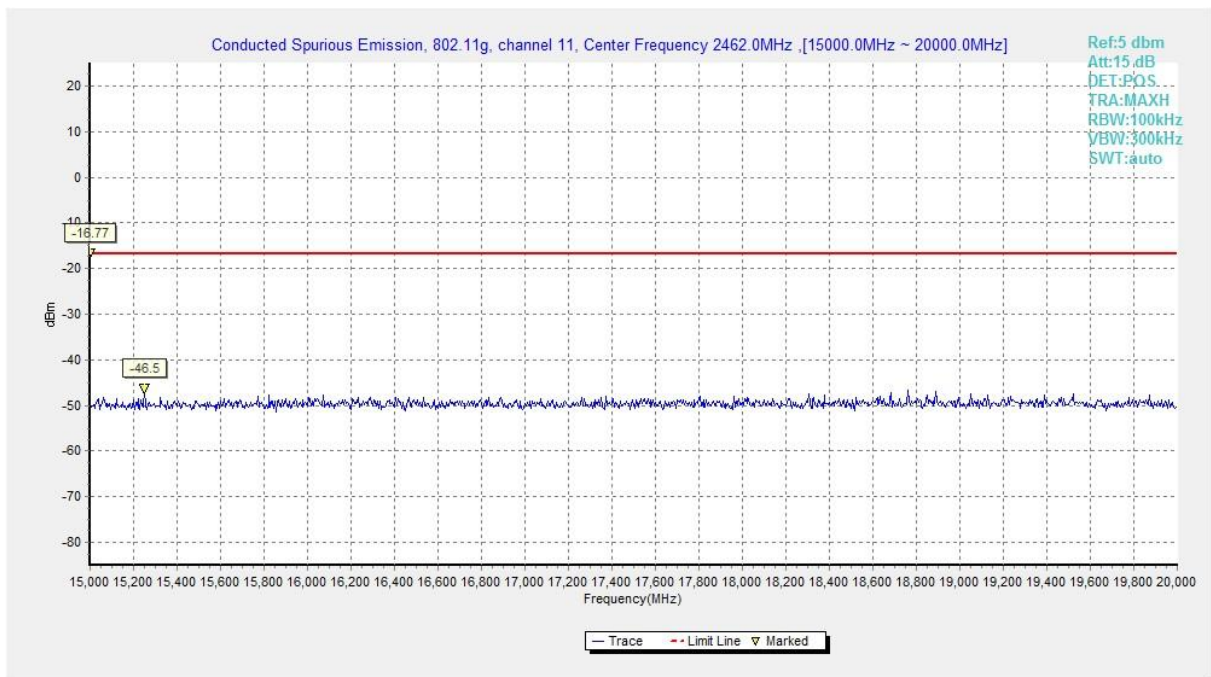
Fig.A.7.1.47 Conducted Spurious Emission (802.11g, Ch11, 15 GHz-20 GHz)
