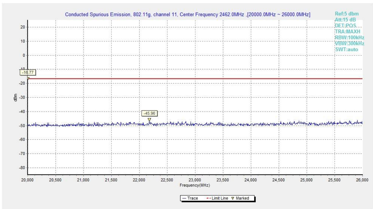
Fig.A.7.1.48 Conducted Spurious Emission (802.11g, Ch11, 20 GHz-26 GHz)
