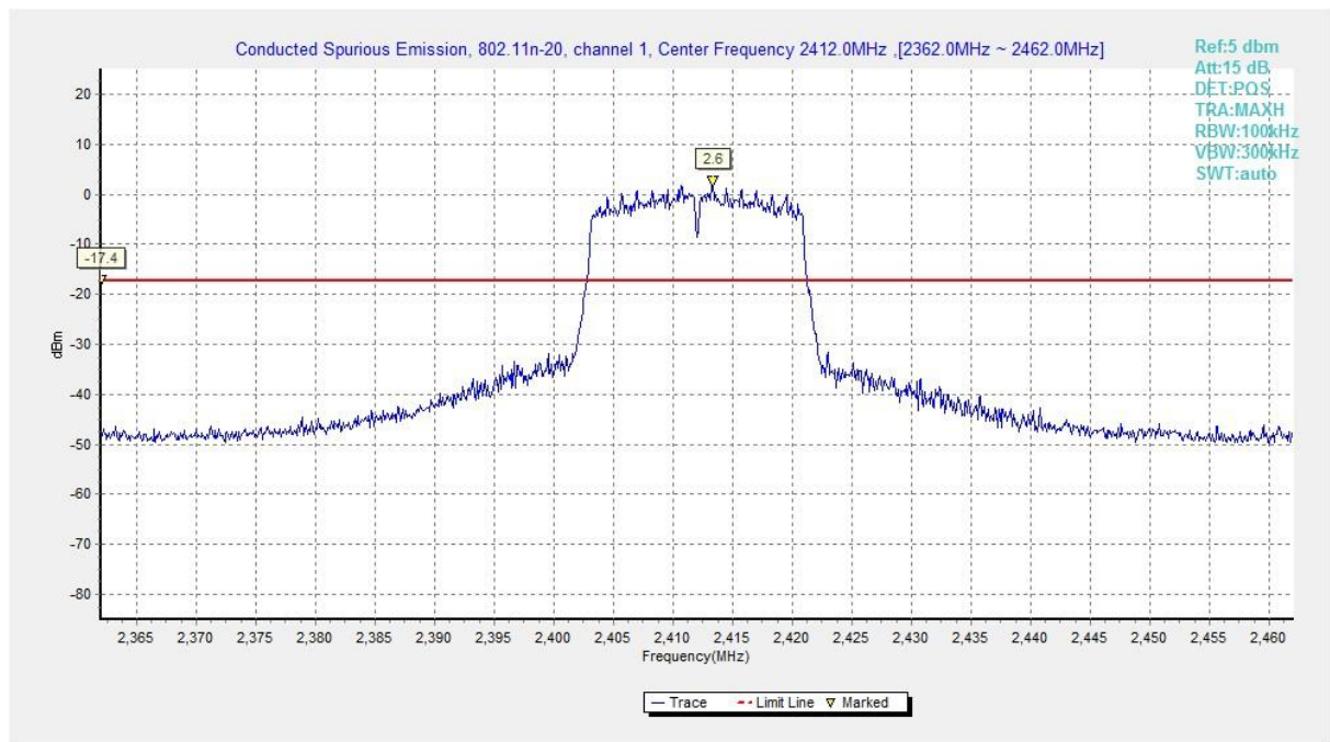
Fig.A.7.1.49 Conducted Spurious Emission (802.11n-HT20, Ch1, Center Frequency)
