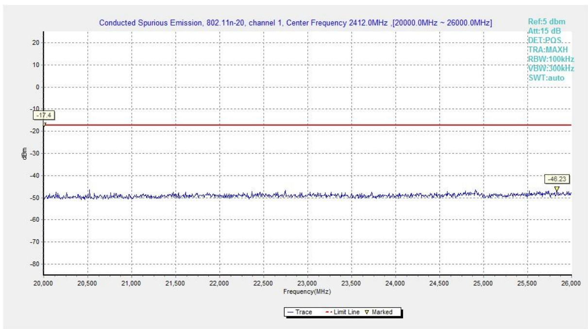
Fig.A.7.1.56 Conducted Spurious Emission (802.11n-HT20, Ch1, 20 GHz-26 GHz)
