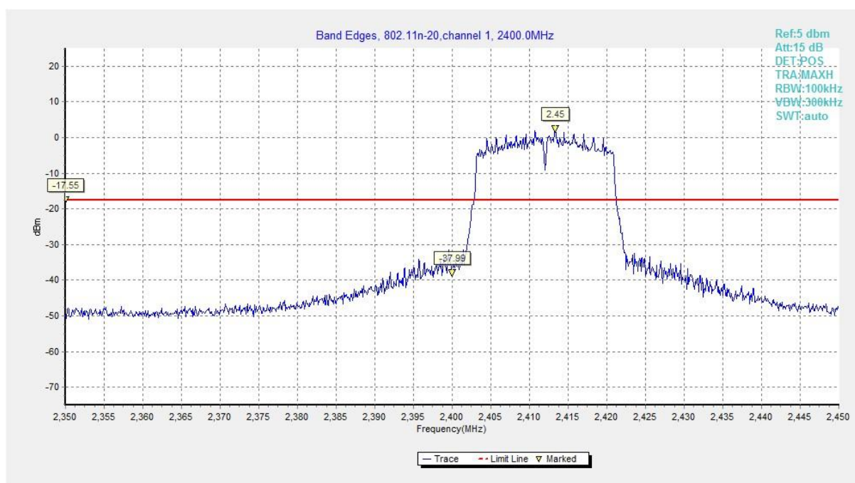
Fig.A.6.5 Band Edges (802.11n-HT20, Ch 1)
