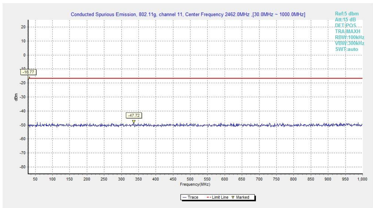
Fig.A.7.1.42 Conducted Spurious Emission (802.11g, Ch11, 30 MHz-1 GHz)
