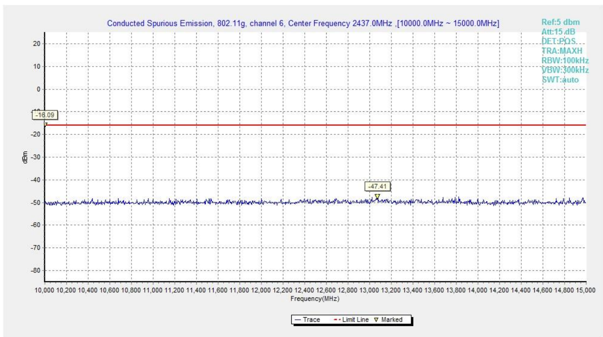
Fig.A.7.1.38 Conducted Spurious Emission (802.11g, Ch6, 10 GHz-15 GHz)
