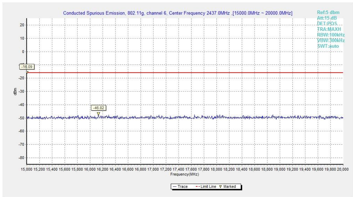
Fig.A.7.1.39 Conducted Spurious Emission (802.11g, Ch6, 15 GHz-20 GHz)
