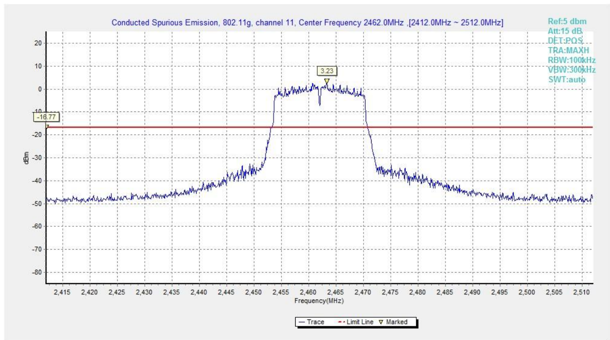
Fig.A.7.1.41 Conducted Spurious Emission (802.11g, Ch11, Center Frequency)
