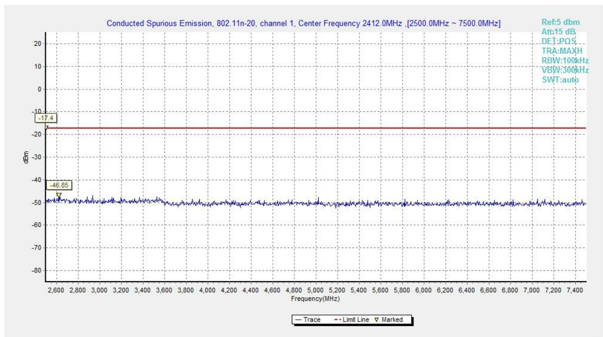
Fig.A.7.1.52 Conducted Spurious Emission (802.11n-HT20, Ch1, 2.5 GHz-7.5 GHz)
