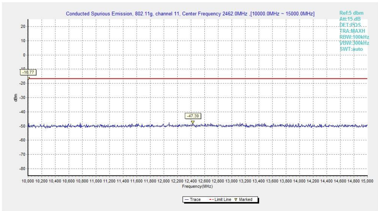
Fig.A.7.1.46 Conducted Spurious Emission (802.11g, Ch11, 10 GHz-15 GHz)
