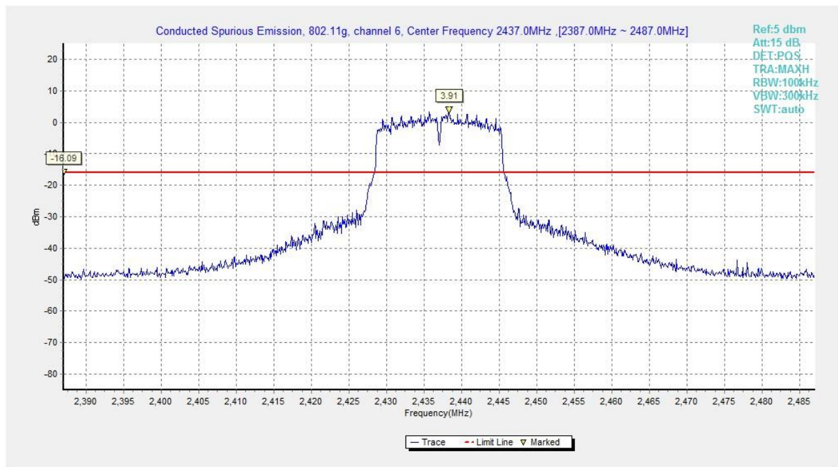
Fig.A.7.1.33 Conducted Spurious Emission (802.11g, Ch6, Center Frequency)
