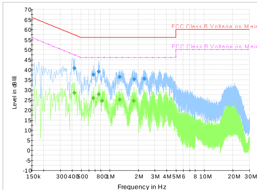
Fig.A.9.2 AC Powerline Conducted Emission-Idle
