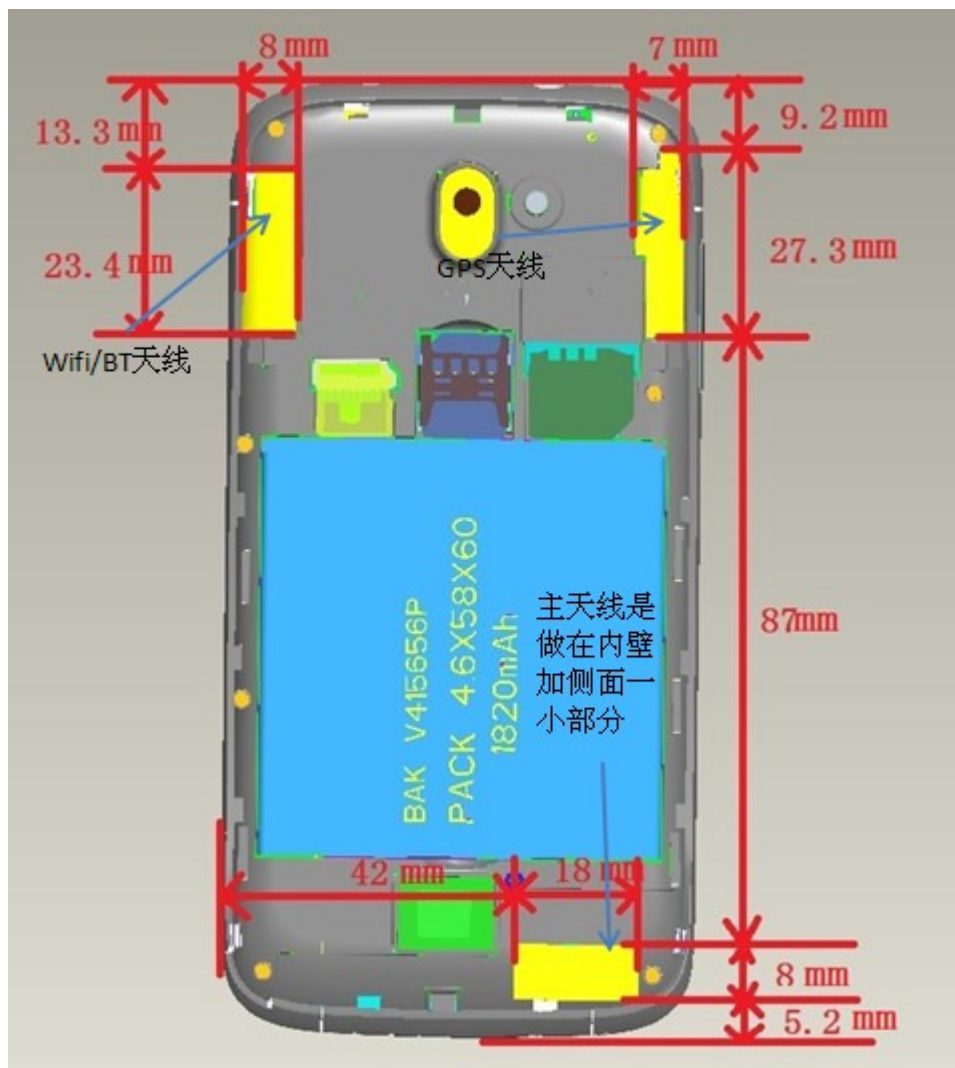
c: Antenna
