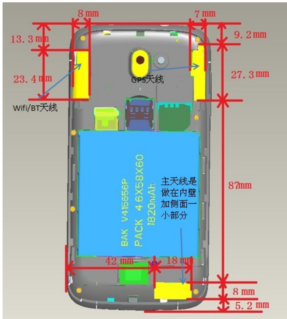
c: Antenna
