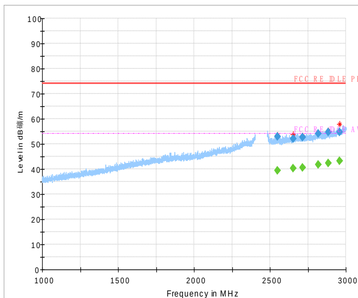
Fig.41 Radiated emission: GFSK, Ch0, 1GHz~3GHz
