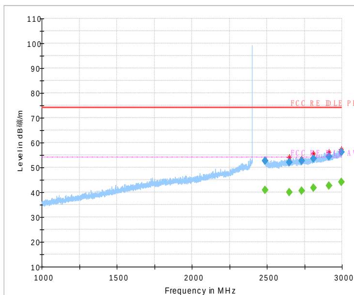
Fig.47 Radiated emission: \pi/4 DQPSK, Ch0, 1GHz~3GHz
