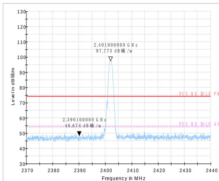
Fig.43 Radiated emission (Power): GFSK, low channel (peak)
