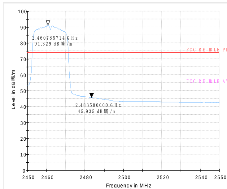
Fig 68. Radiated emission (Power): 802.11n, high channel
