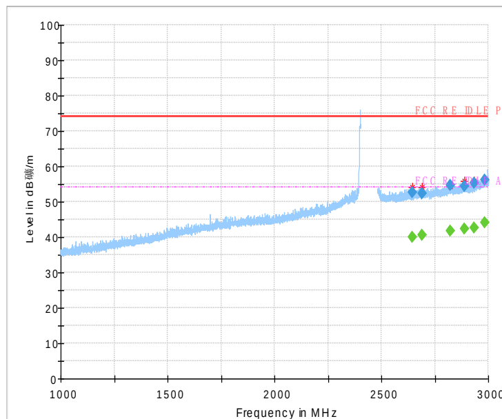
Fig 60. Radiated Spurious Emission (802.11b,Ch1,1GHz~3GHz)
