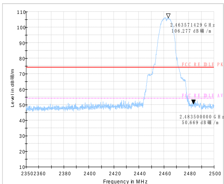
Fig 58. Radiated emission (Power): 802.11b, high channel
