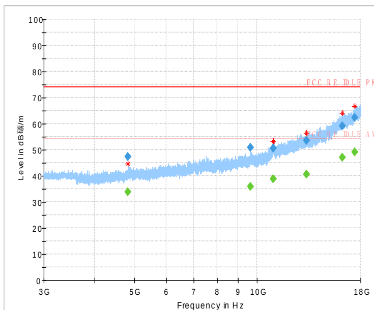
Fig 66. Radiated Spurious Emission (802.11g,Ch11,3GHz~18GHz)
