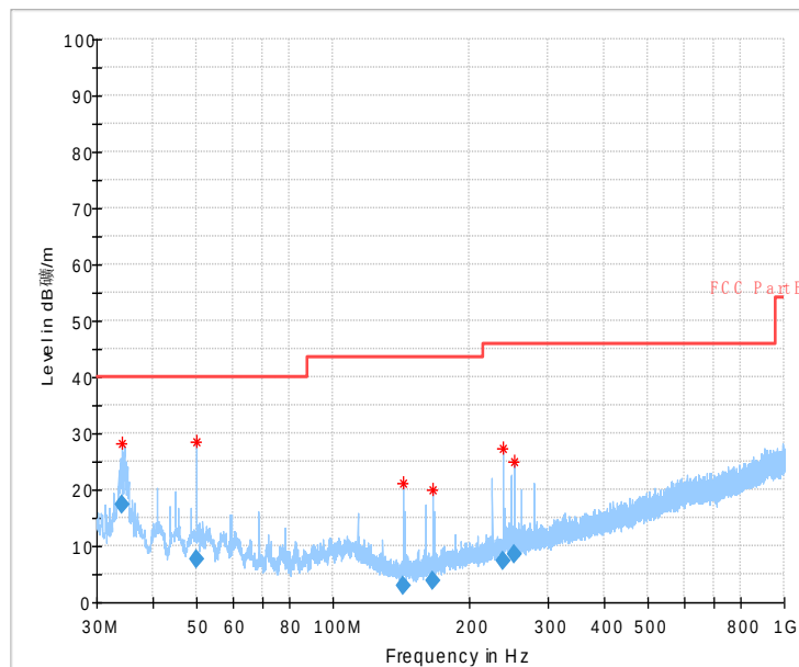
Fig 64. Radiated Spurious Emission (802.11g, Ch11, 30MHz~1GHz)
