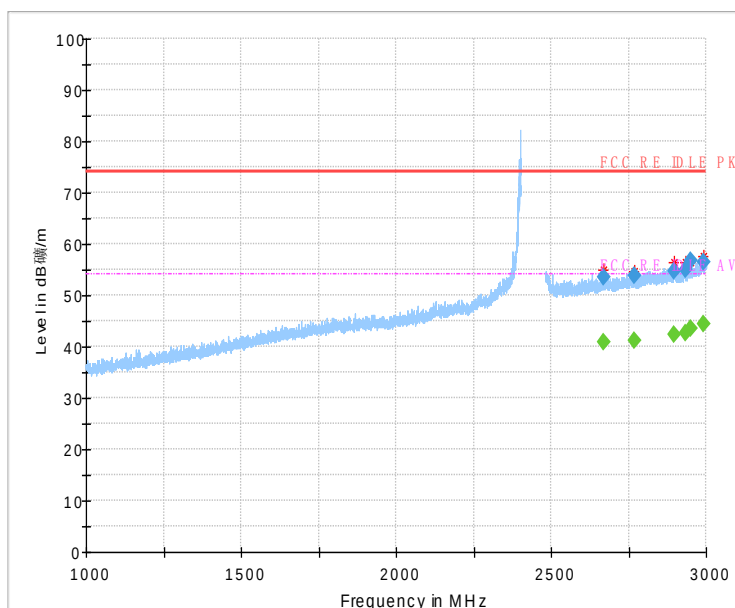
Fig 65. Radiated Spurious Emission (802.11g,Ch11,1GHz~3GHz)
