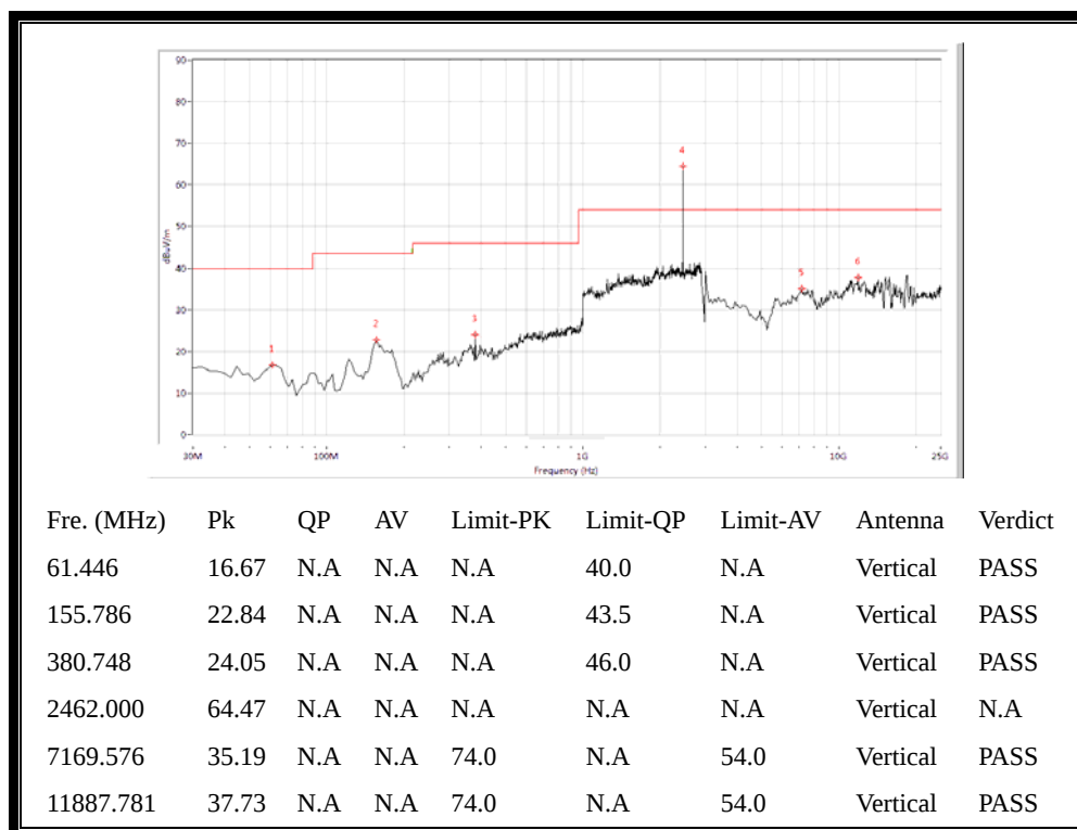
(Plot F.3: Antenna Vertical, 30MHz to 25GHz)
