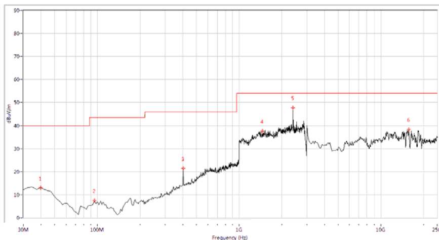
(Plot A.1: 30MHz to 25GHz, Antenna Horizontal @ □/4-DQPSK, channel 0)
