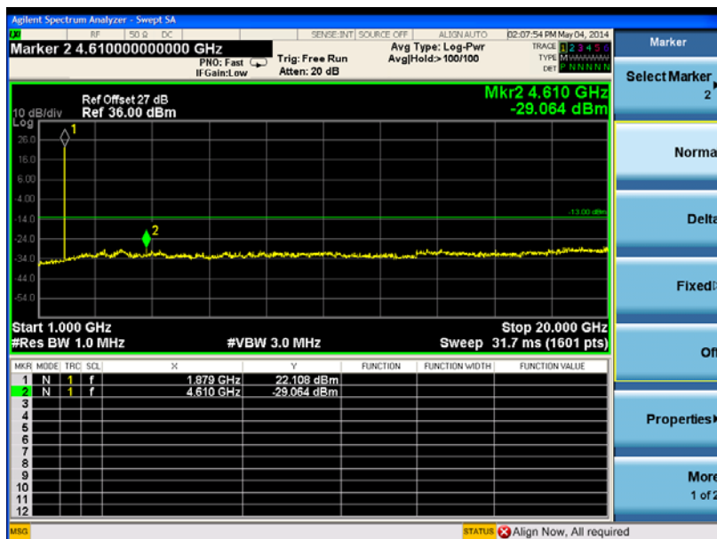
(Plot K2.1: HSPA+ 1900MHz Channel = 9400, 1GHz to 20GHz)
