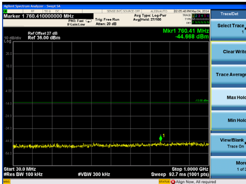
(Plot K 2: HSPA+ 1900MHz Channel = 9400, 30MHz to 1GHz)
