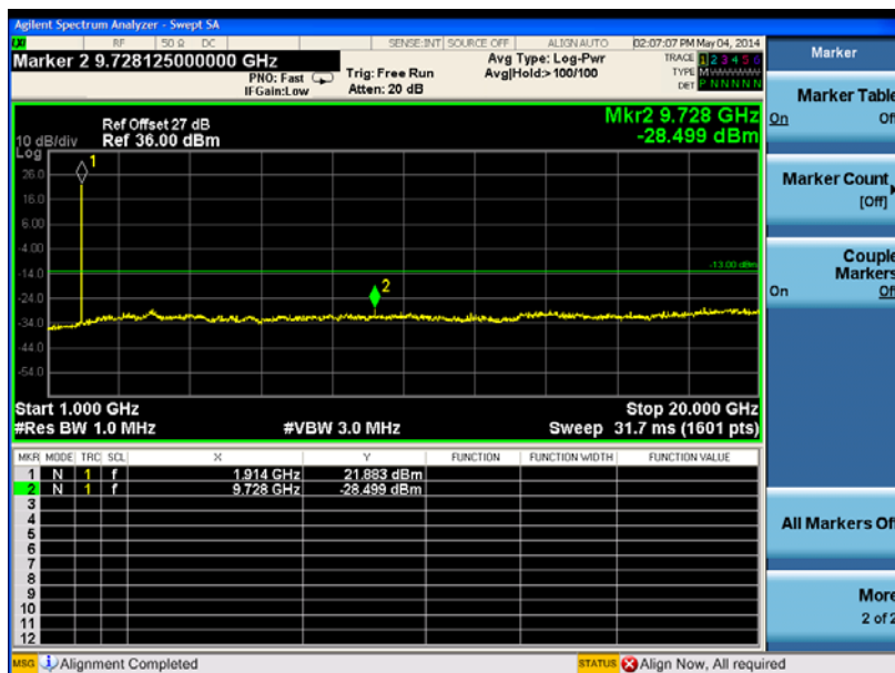
(Plot K3.1: HSPA+ 1900MHz Channel = 9538 1GHz to 20GHz)
