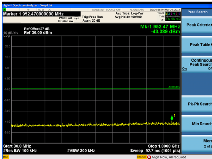
(Plot K 3: HSPA+ 1900MHz Channel = 9538, 30MHz to 1GHz)
