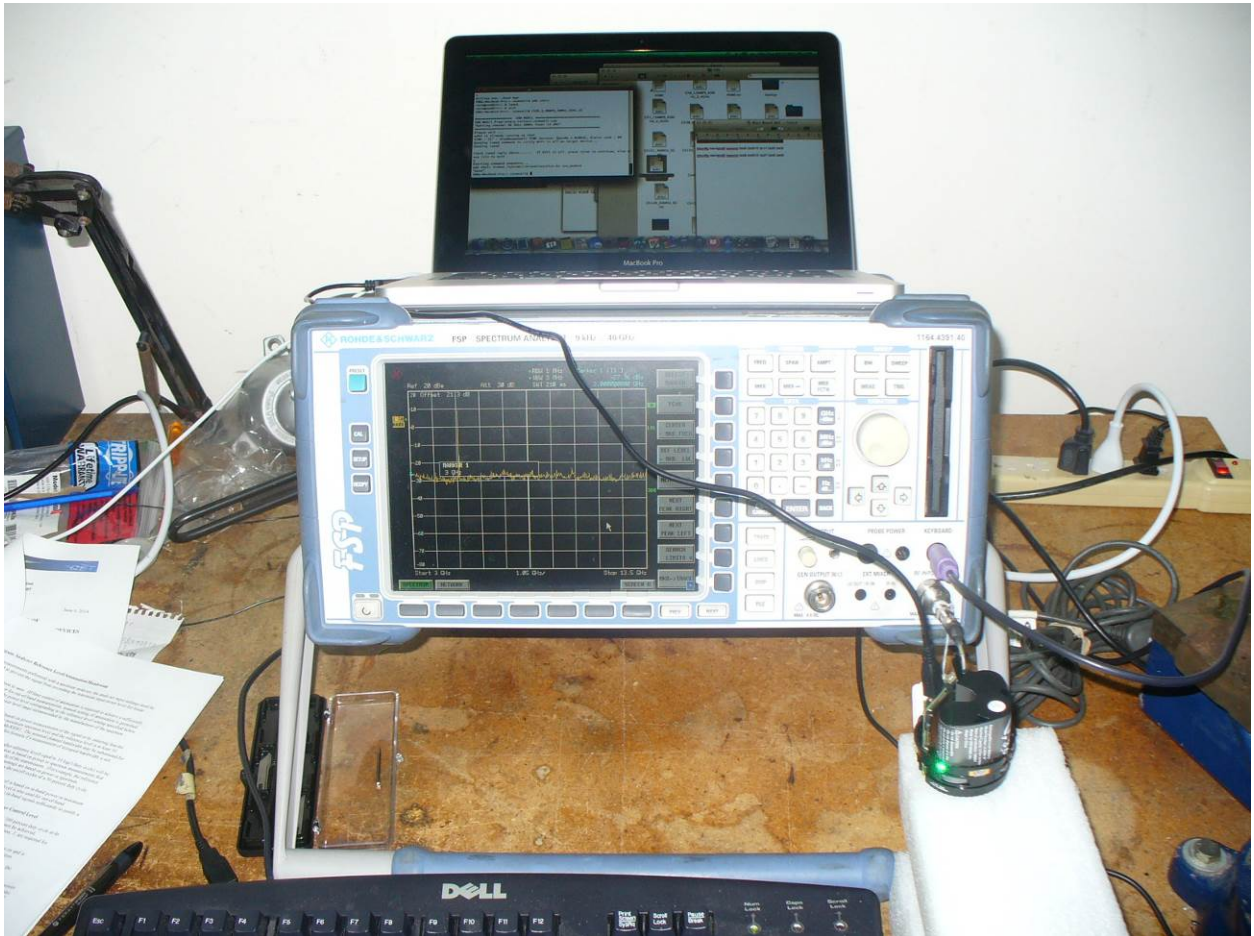
Figure 4: RF Conducted Test Setup – FCC 15.407
