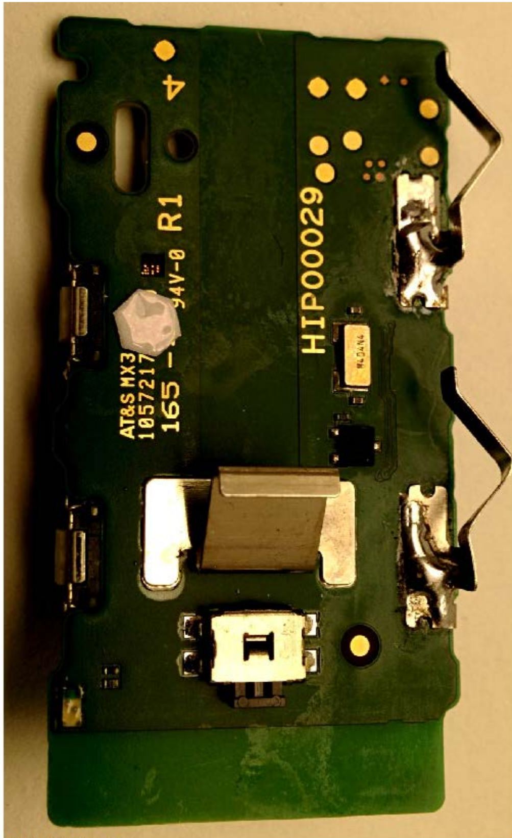
Figure 2: PCB View 2
