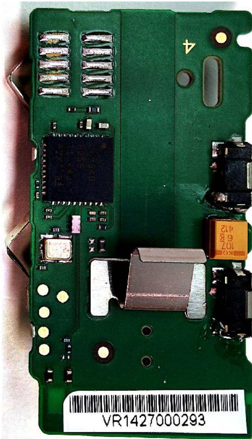
Figure 1: PCB View 1
