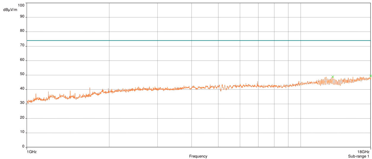
Plot 17: Radiated Spurious Emissions Requirements, Mid Channel, Peak (Chip Antenna)
