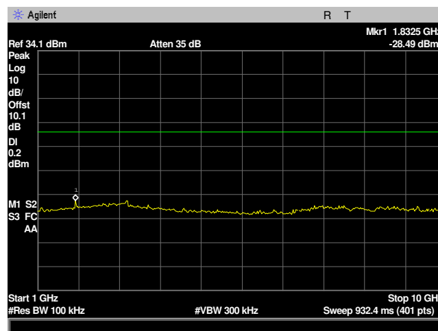
Plot 26: RF Conducted Spurious Emissions Requirements, 1GHz-10GHz Mid Channel
