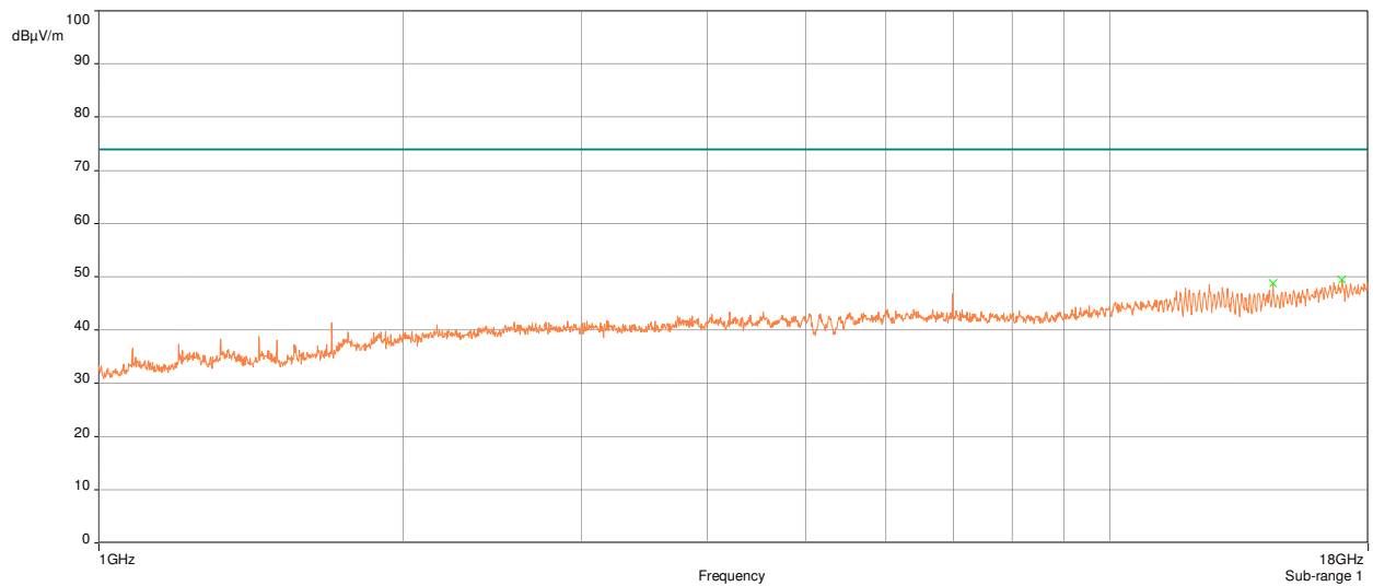
Plot 19: Radiated Spurious Emissions Requirements, High Channel, Peak (Chip Antenna)
