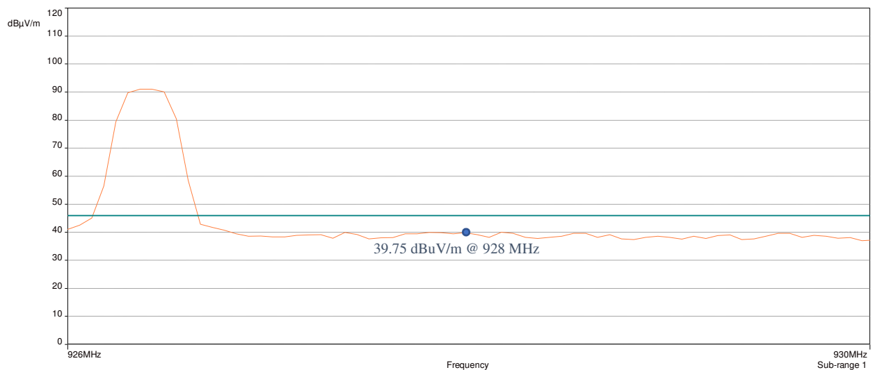
Plot 21: Radiated Band Edge, High Channel, Chip, Worst Case
