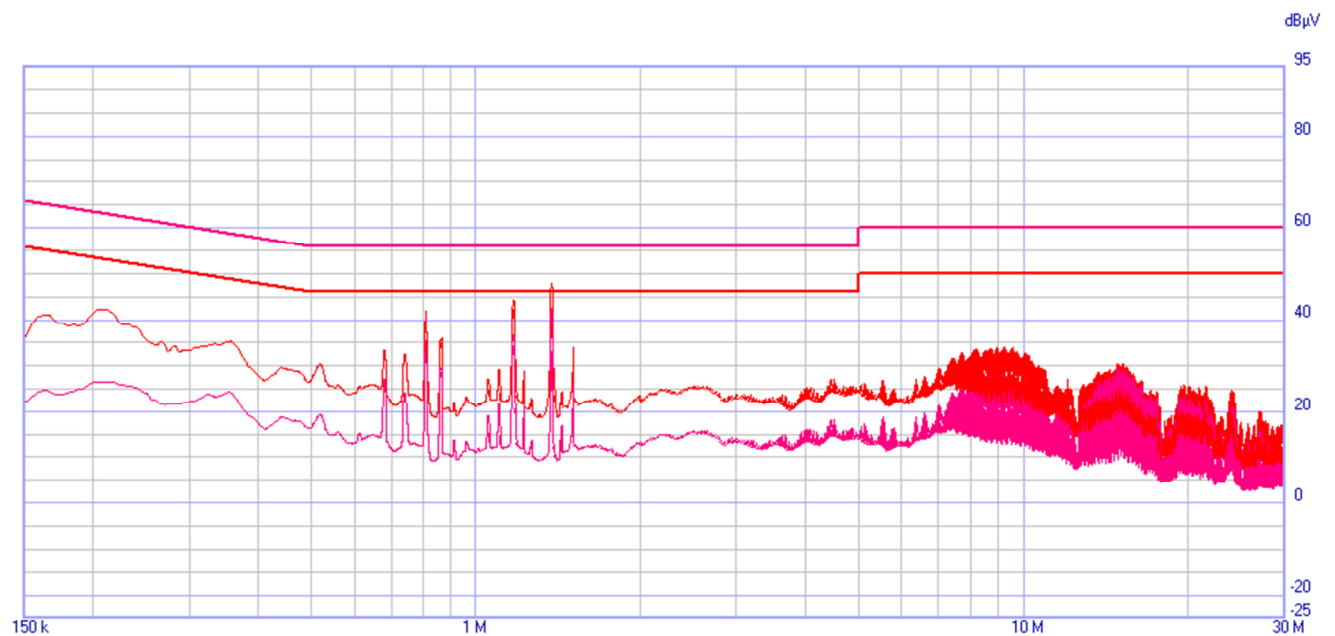
Plot 1. Conducted Emission, Line Plot - Chip Antenna
