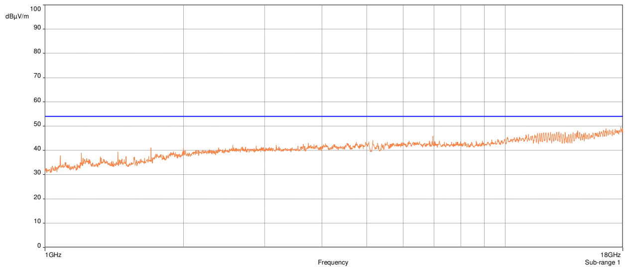
Plot 16: Radiated Spurious Emissions Requirements, Mid Channel, Average (Chip Antenna)
