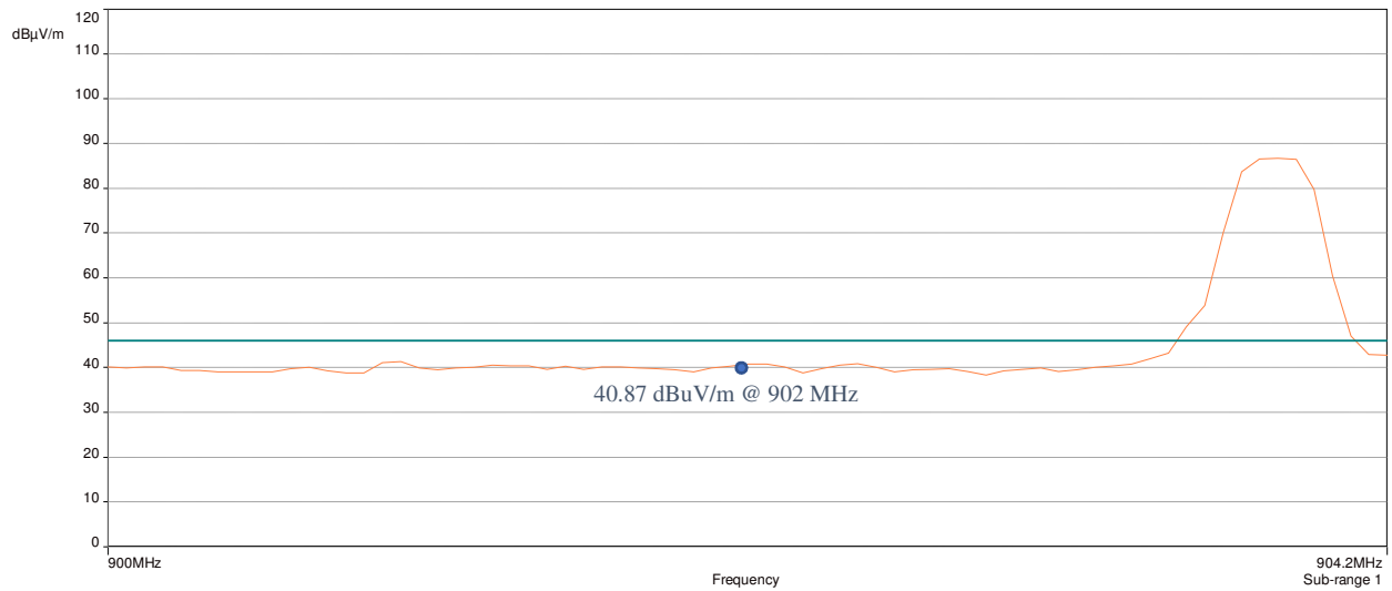
Plot 20: Radiated Band Edge, Low Channel, Chip, Worst Case
