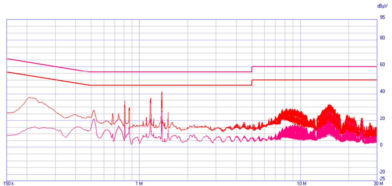
Plot 2. Conducted Emission, Neutral Plot – Chip Antenna
