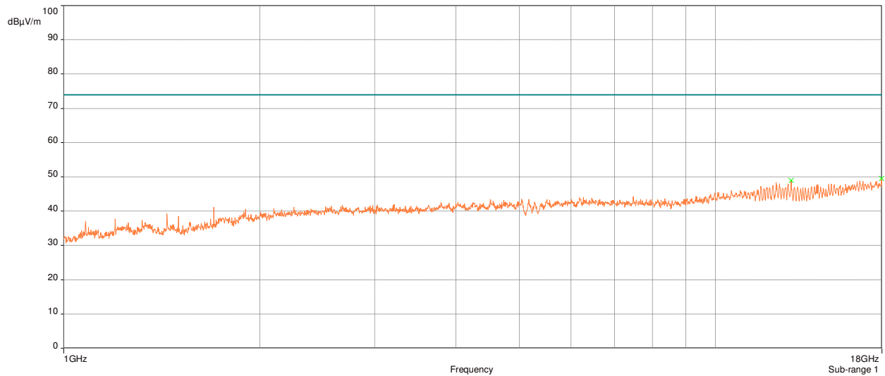
Plot 15: Radiated Spurious Emissions Requirements, Low Channel, Peak (Chip Antenna)
