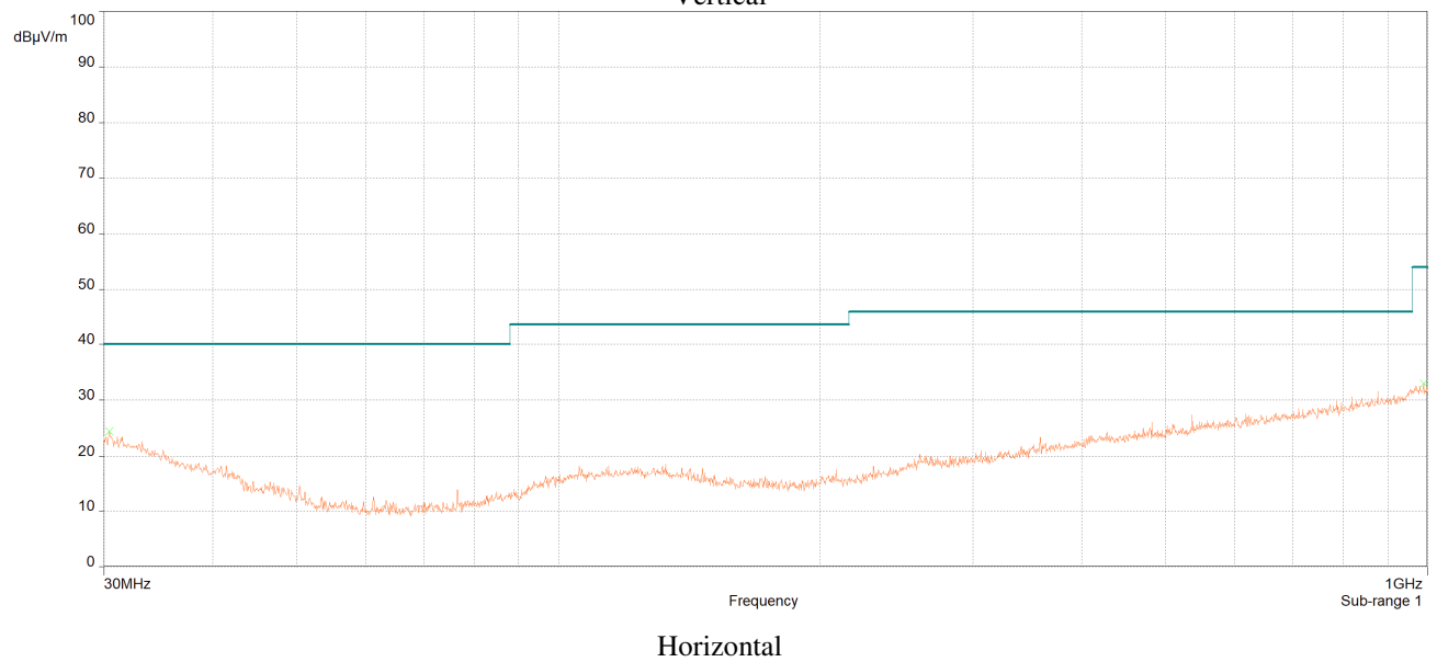
Plot 13: Radiated Emissions, 30 MHz - 1 GHz, (worst case)
