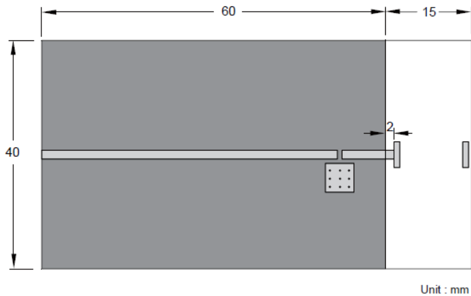
Fig. 2 Outlook and dimension of evaluation board
