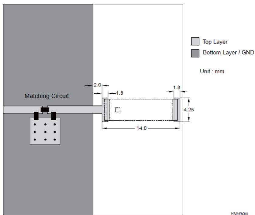
Fig. 3 Details of soldering Pad
