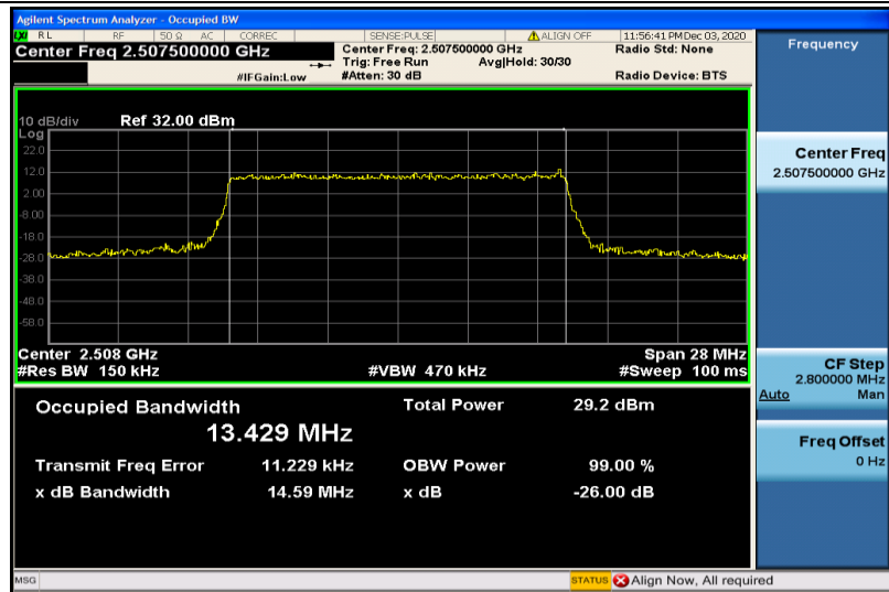
Band7-15MHz-16QAM-20825-75RB#0-13.429
