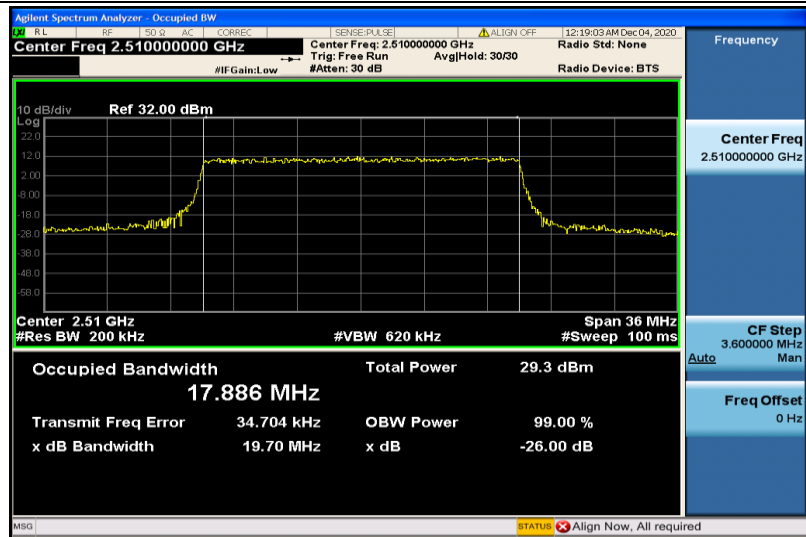
Band7-20MHz-16QAM-20850-100RB#0-17.886
