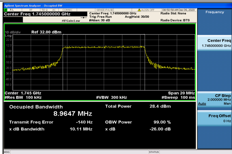
Band66-10MHz-16QAM-132322-50RB#0-8.9647
