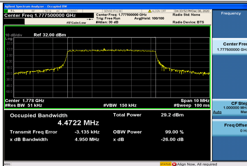
Band66-5MHz-16QAM-132647-25RB#0-4.4722
