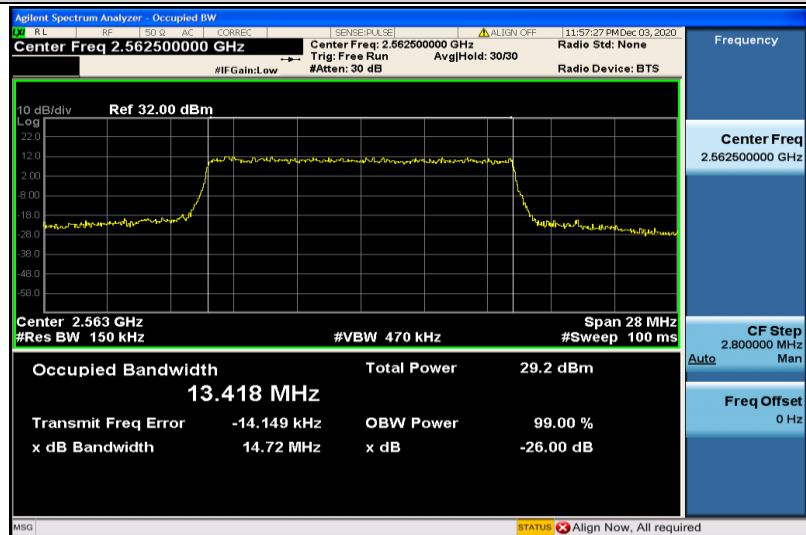
Band7-15MHz-16QAM-21375-75RB#0-13.418
