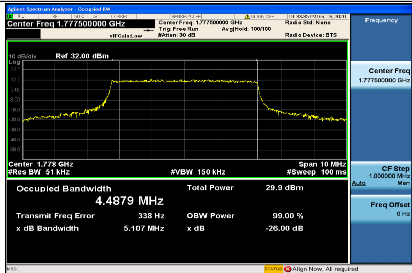
Band66-5MHz-QPSK-132647-25RB#0-4.4879
