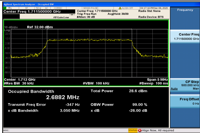
Band66-3MHz-16QAM-131987-15RB#0-2.6882
