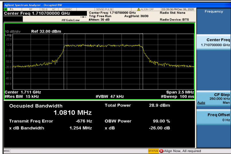
Band66-1.4MHz-QPSK-131979-6RB#0-1.0810
