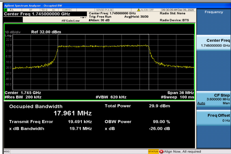
Band66-20MHz-QPSK-132322-100RB#0-17.961
