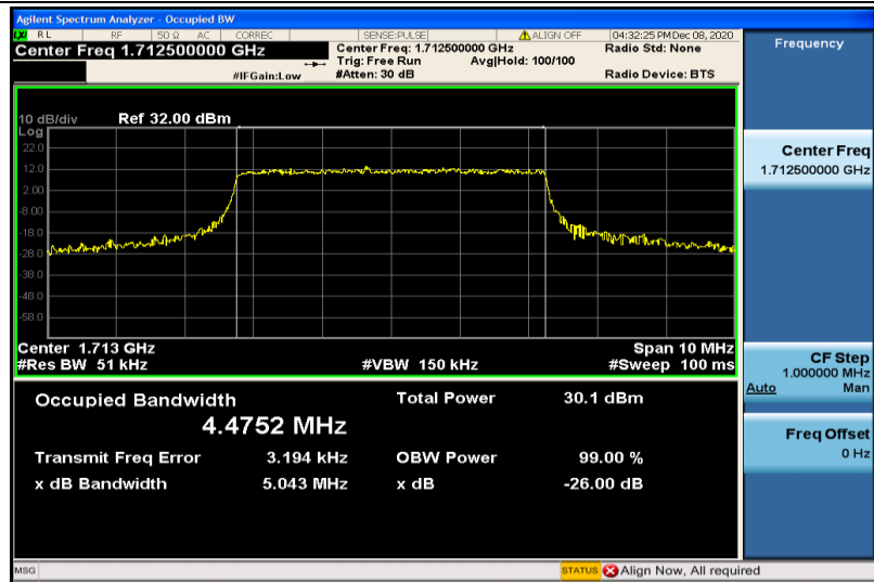
Band66-5MHz-QPSK-131997-25RB#0-4.4752
