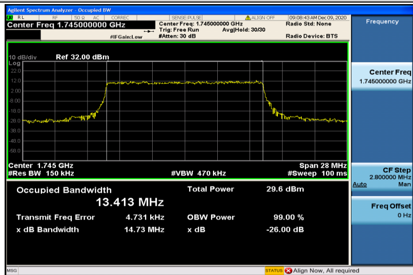
Band66-15MHz-QPSK-132322-75RB#0-13.413
