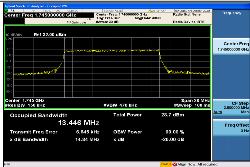
Band66-15MHz-16QAM-132322-75RB#0-13.446
