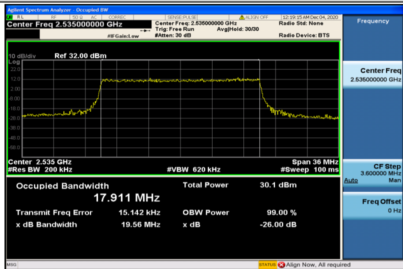
Band7-20MHz-QPSK-21100-100RB#0-17.911
