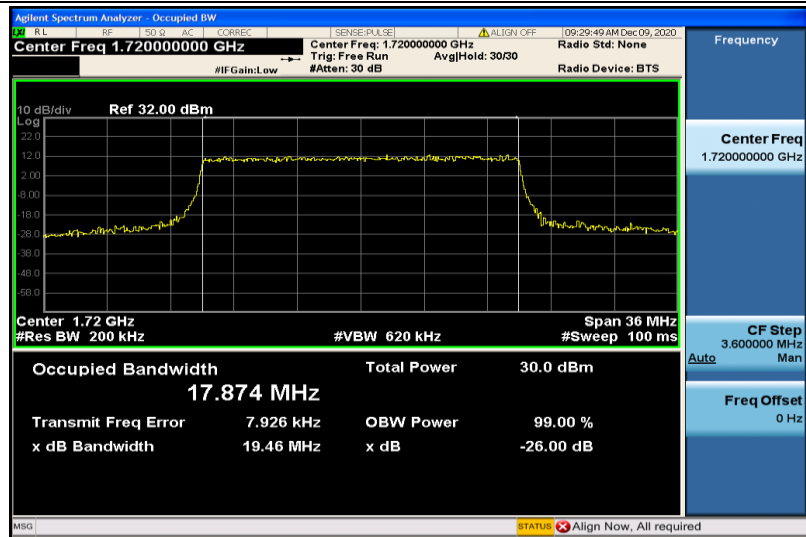
Band66-20MHz-QPSK-132072-100RB#0-17.874
