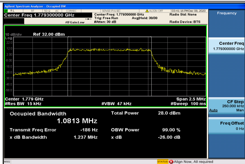
Band66-1.4MHz-16QAM-132665-6RB#0-1.0813
