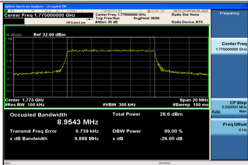
Band66-10MHz-16QAM-132622-50RB#0-8.9543
