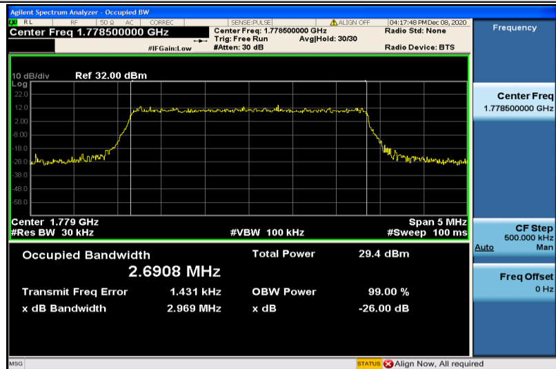
Band66-3MHz-QPSK-132657-15RB#0-2.6908
