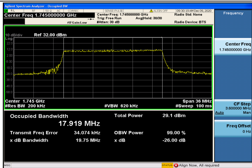
Band66-20MHz-16QAM-132322-100RB#0-17.919
