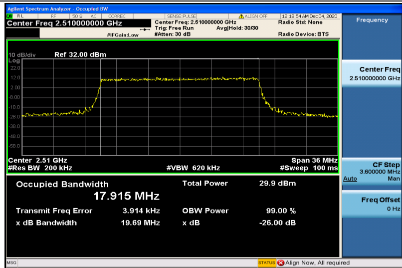
Band7-20MHz-QPSK-20850-100RB#0-17.915
