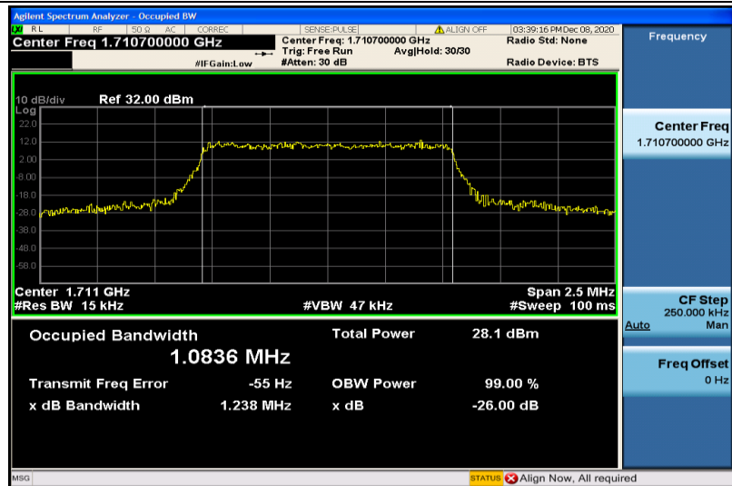
Band66-1.4MHz-16QAM-131979-6RB#0-1.0836
