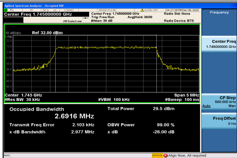
Band66-3MHz-QPSK-132322-15RB#0-2.6916
