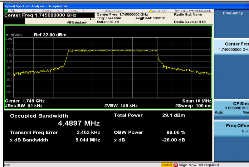
Band66-5MHz-16QAM-132322-25RB#0-4.4897
