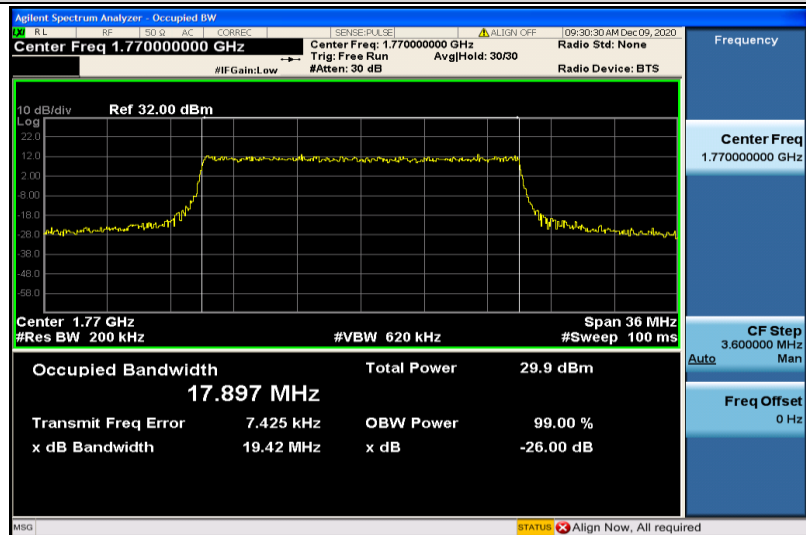
Band66-20MHz-QPSK-132572-100RB#0-17.897
