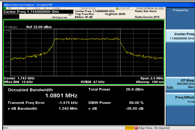
Band66-1.4MHz-QPSK-132322-6RB#0-1.0801
