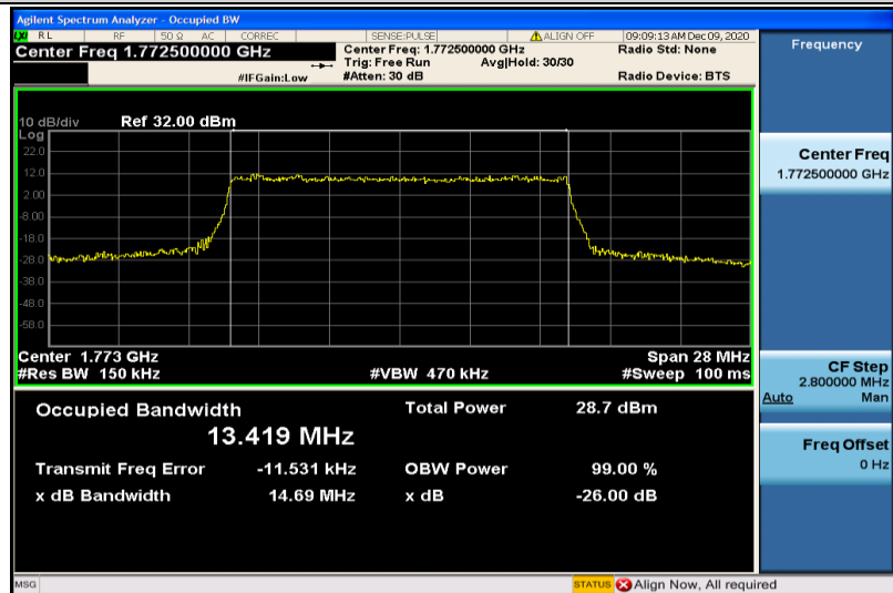
Band66-15MHz-16QAM-132597-75RB#0-13.419
