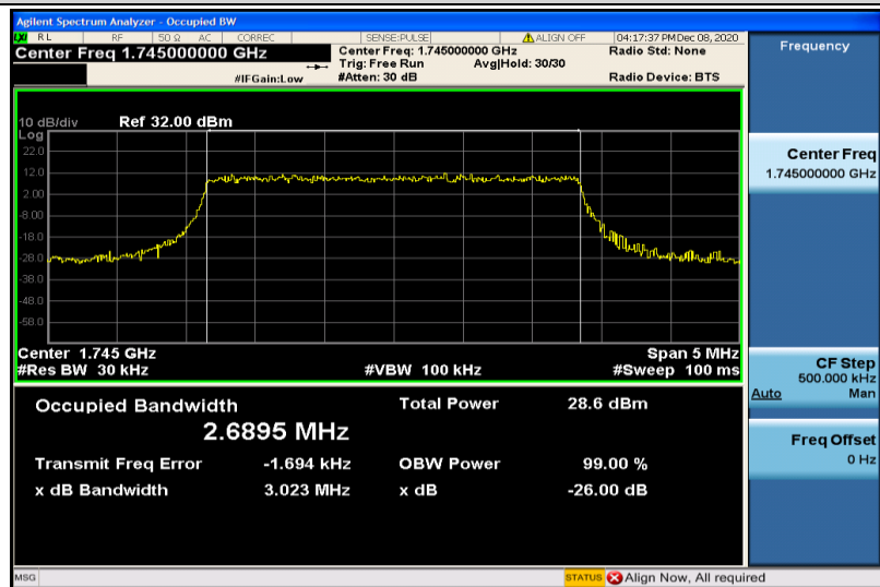
Band66-3MHz-16QAM-132322-15RB#0-2.6895
