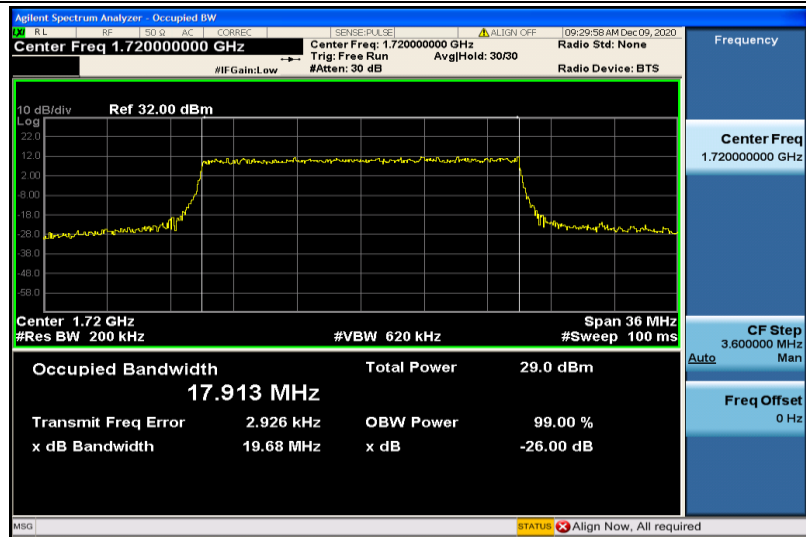
Band66-20MHz-16QAM-132072-100RB#0-17.913
