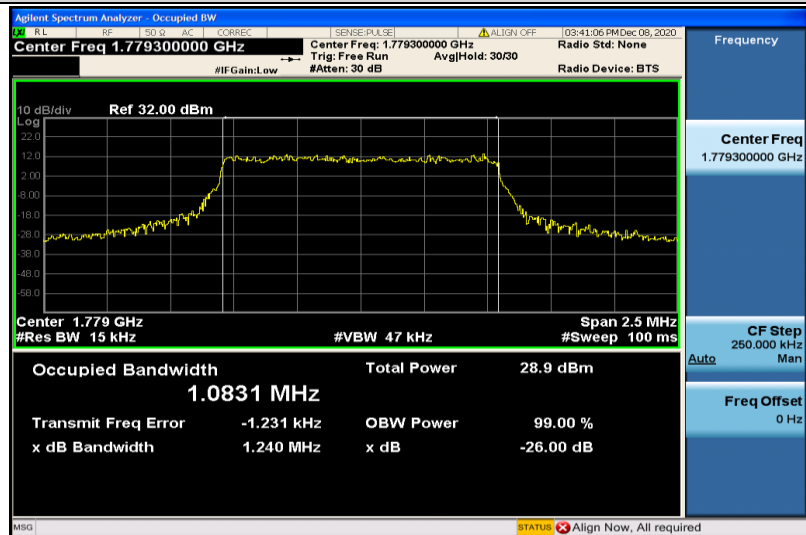
Band66-1.4MHz-QPSK-132665-6RB#0-1.0831
