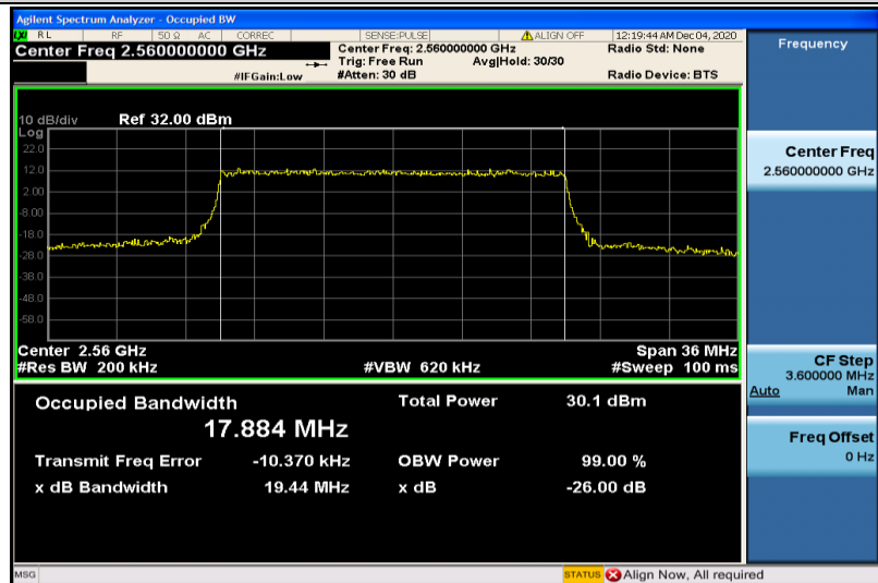
Band7-20MHz-QPSK-21350-100RB#0-17.884
