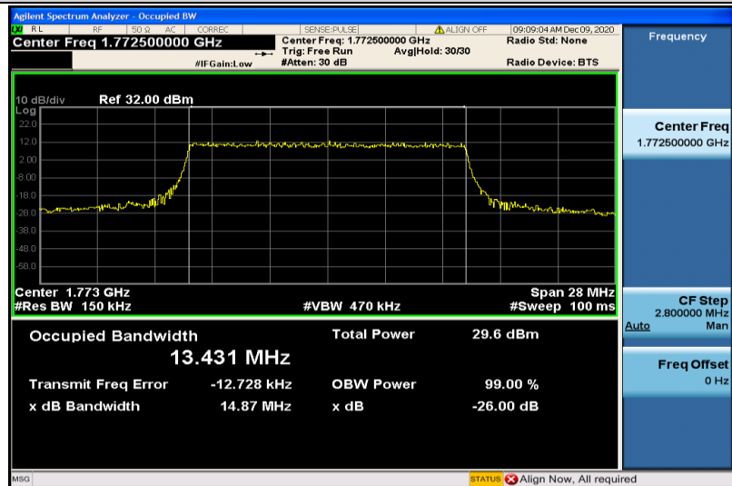
Band66-15MHz-QPSK-132597-75RB#0-13.431
