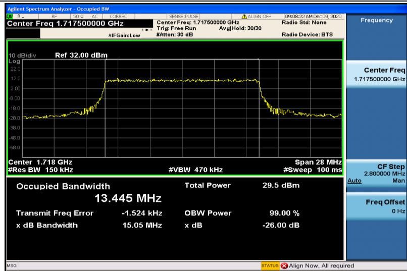
Band66-15MHz-QPSK-132047-75RB#0-13.445
