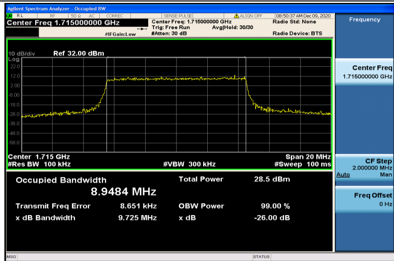
Band66-10MHz-16QAM-132022-50RB#0-8.9484
