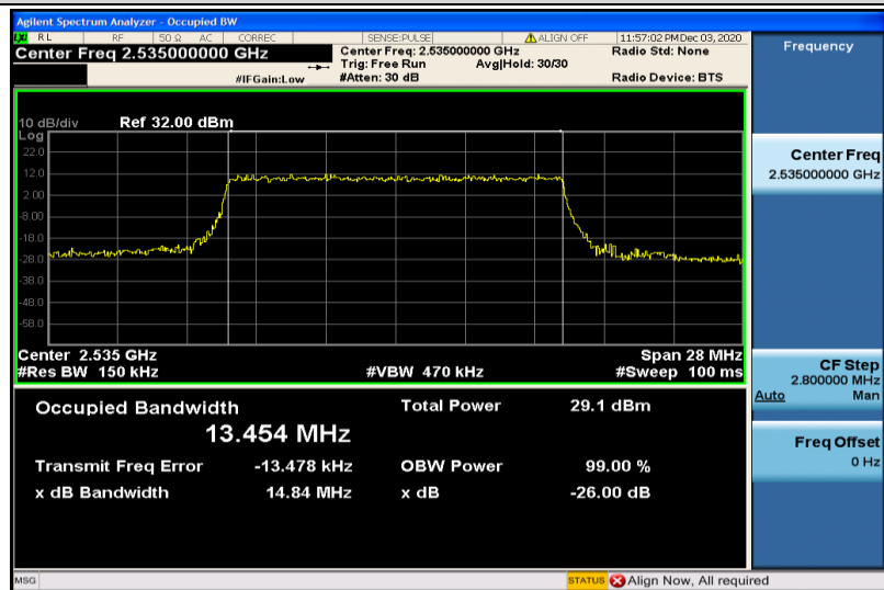
Band7-15MHz-16QAM-21100-75RB#0-13.454
