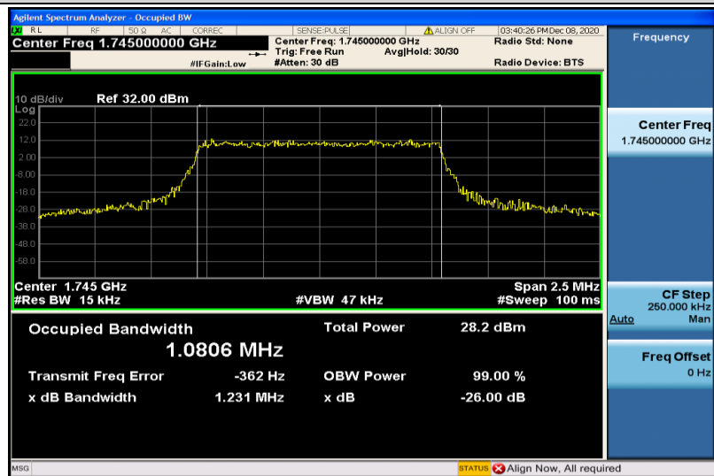
Band66-1.4MHz-16QAM-132322-6RB#0-1.0806
