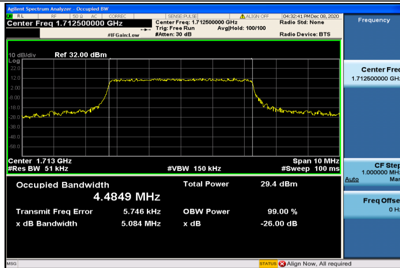
Band66-5MHz-16QAM-131997-25RB#0-4.4849
