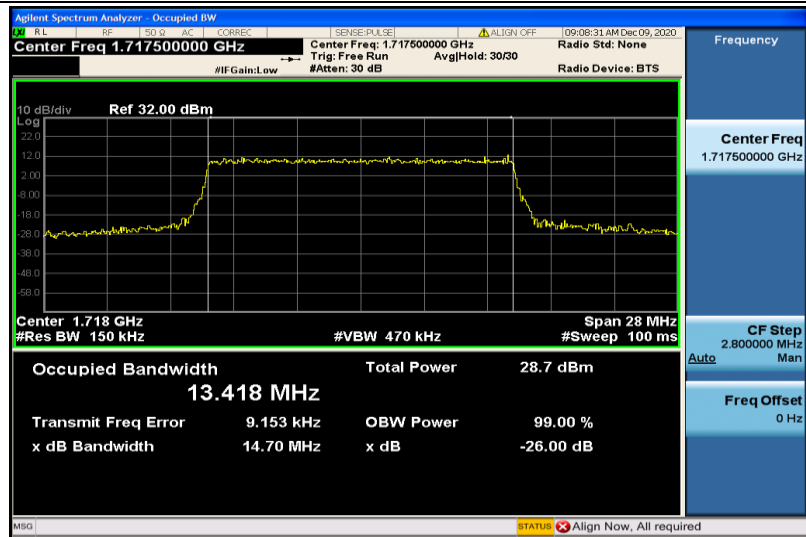
Band66-15MHz-16QAM-132047-75RB#0-13.418
