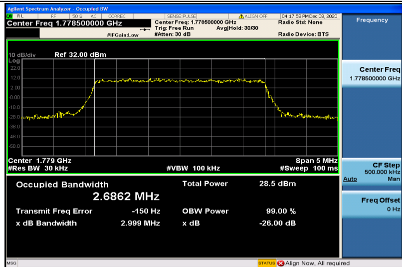
Band66-3MHz-16QAM-132657-15RB#0-2.6862
