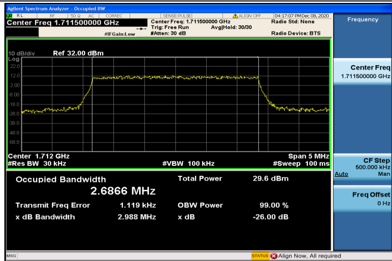
Band66-3MHz-QPSK-131987-15RB#0-2.6866
