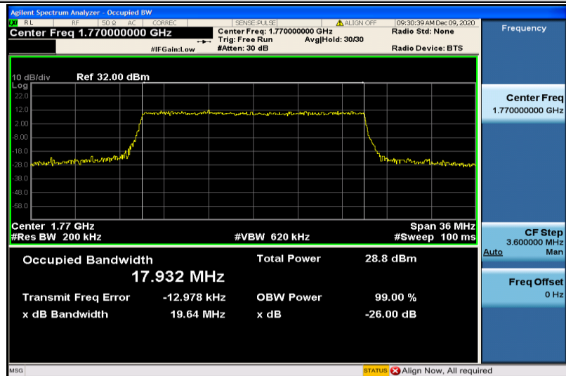
Band66-20MHz-16QAM-132572-100RB#0-17.932
