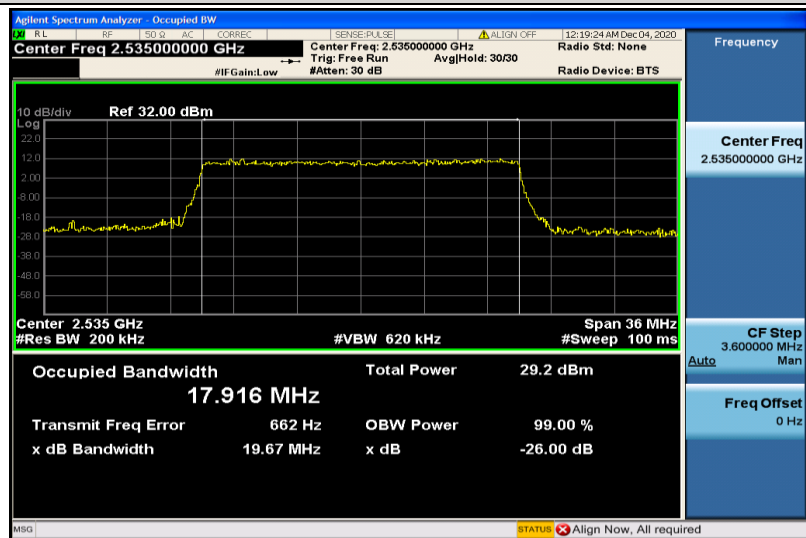
Band7-20MHz-16QAM-21100-100RB#0-17.916
