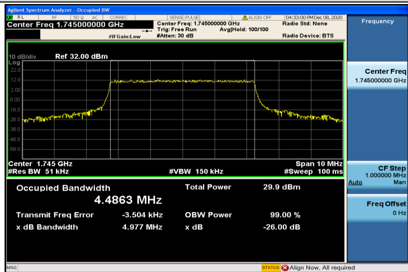
Band66-5MHz-QPSK-132322-25RB#0-4.4863
