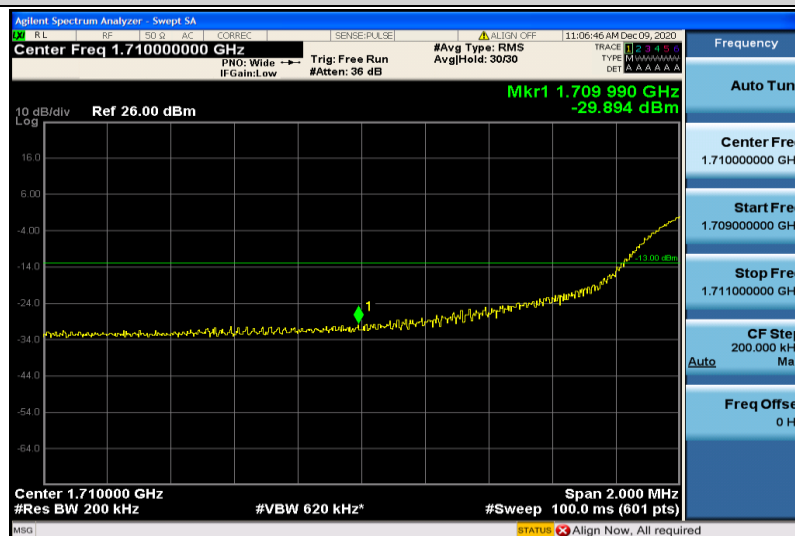
Band66-20MHz-QPSK-132072-100RB#0
