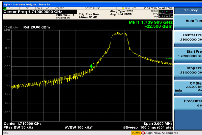
Band66-3MHz-16QAM-131987-1RB#0
