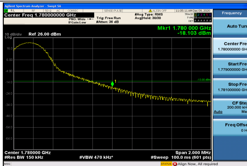
Band66-15MHz-QPSK-132597-1RB#74
