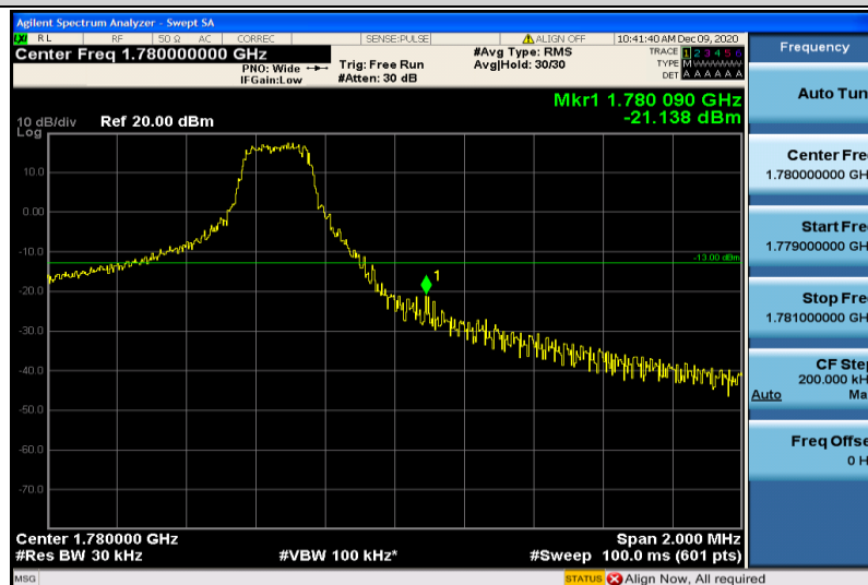
Band66-3MHz-16QAM-132657-1RB#14
