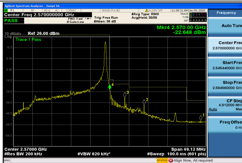
Band7-20MHz-16QAM-21350-1RB#99
