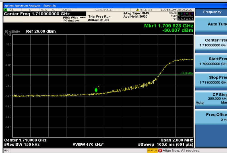
Band66-15MHz-16QAM-132047-75RB#0
