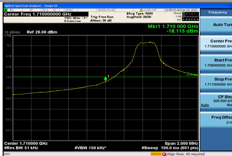
Band66-5MHz-QPSK-131997-1RB#0
