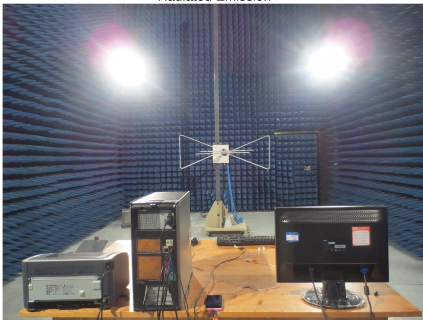
Radiated Emission
