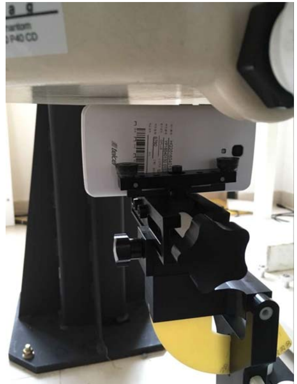
Hotspot mode - Right Side (10mm)
