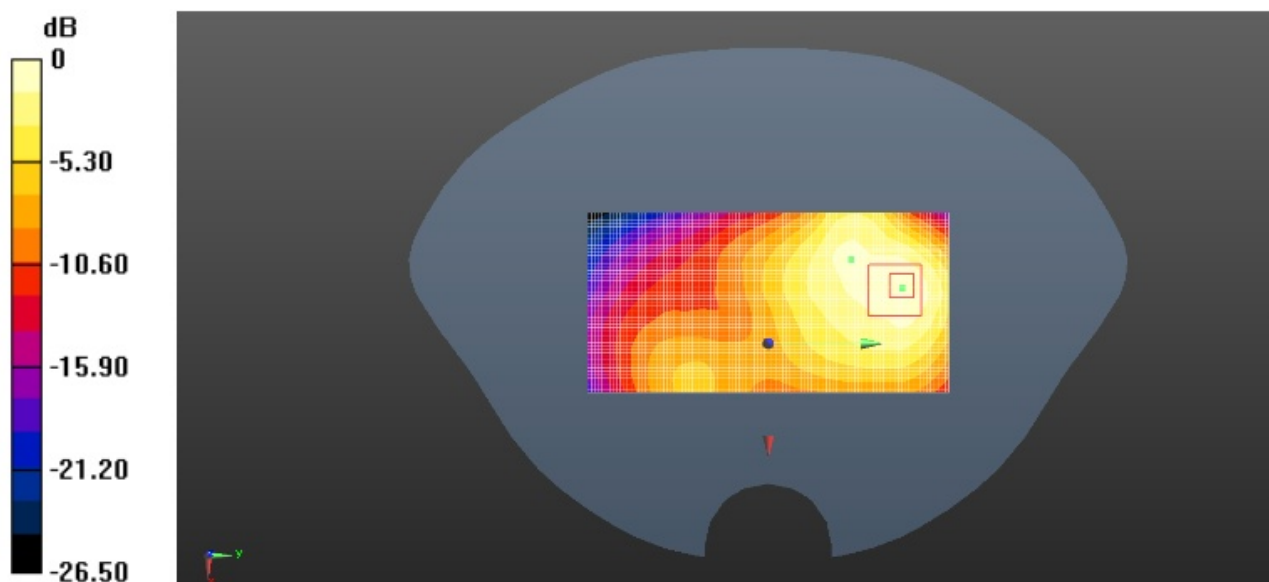
Body- worn Rear Side (PCS1900 Middle Channel)
