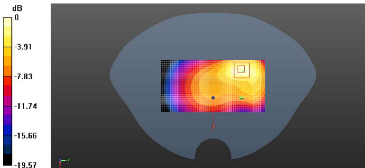
Body- worn Rear Side (GSM850 Middle Channel)
