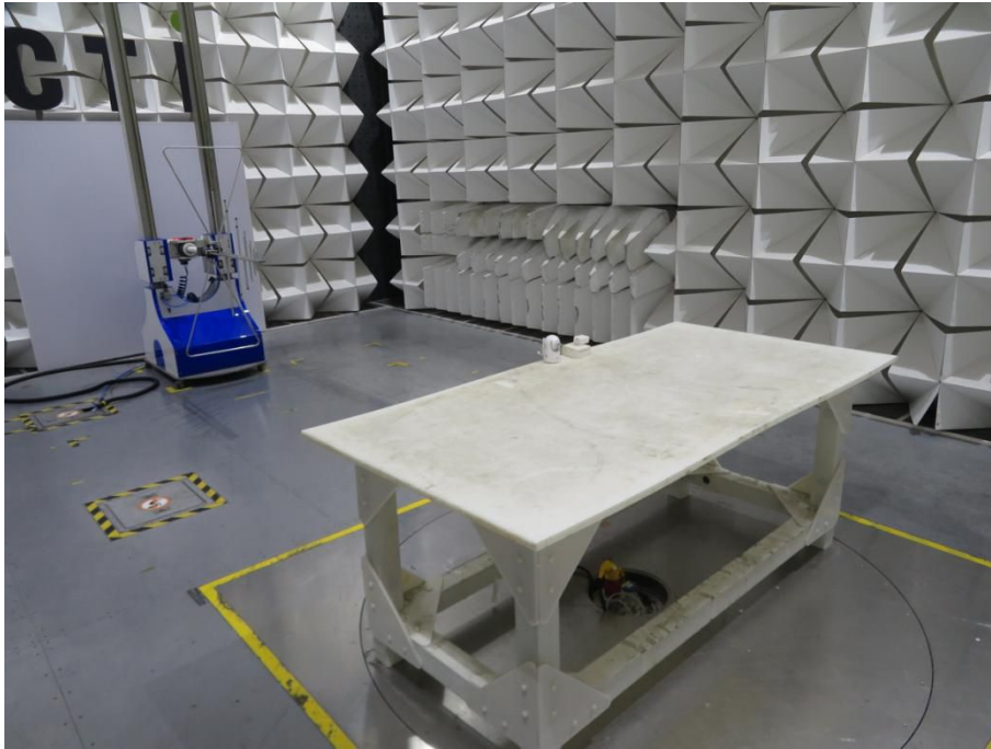
Adapter 1: BLJ06W059100P1-U
