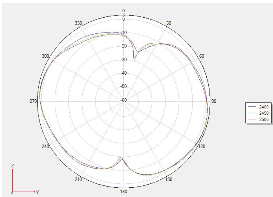
Phi 90 2D
