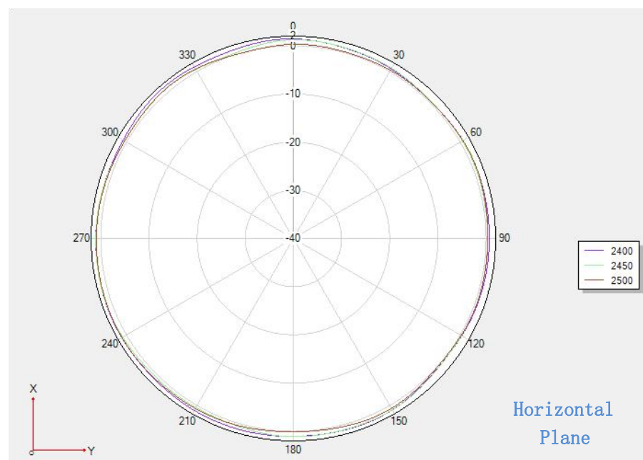
Theta 90 2D
