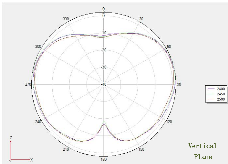
Phi 0 2D
