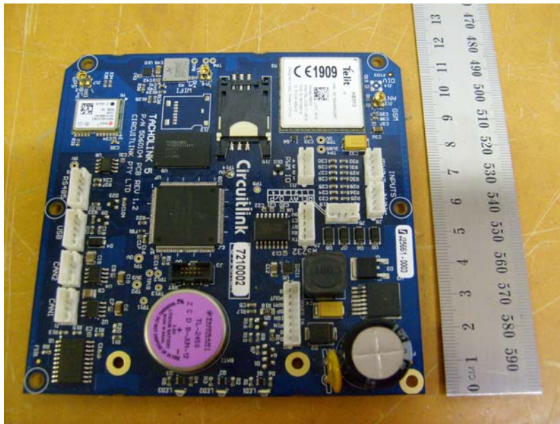
TACHO5C Main PCB (Component Side)
