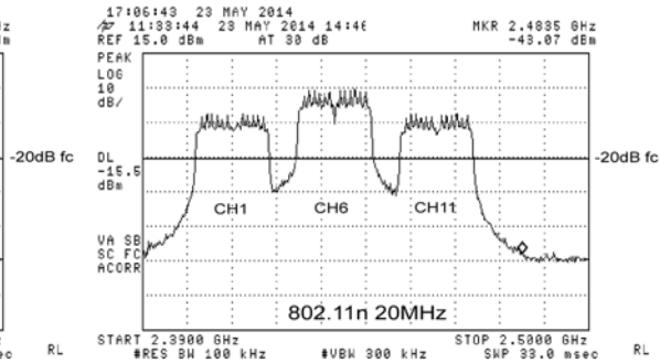
Band-edges
