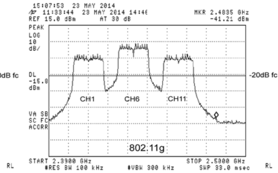
Band-edges
